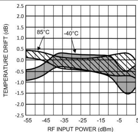
Figure 74. Temperature Drift Error without Temperature Compensation
