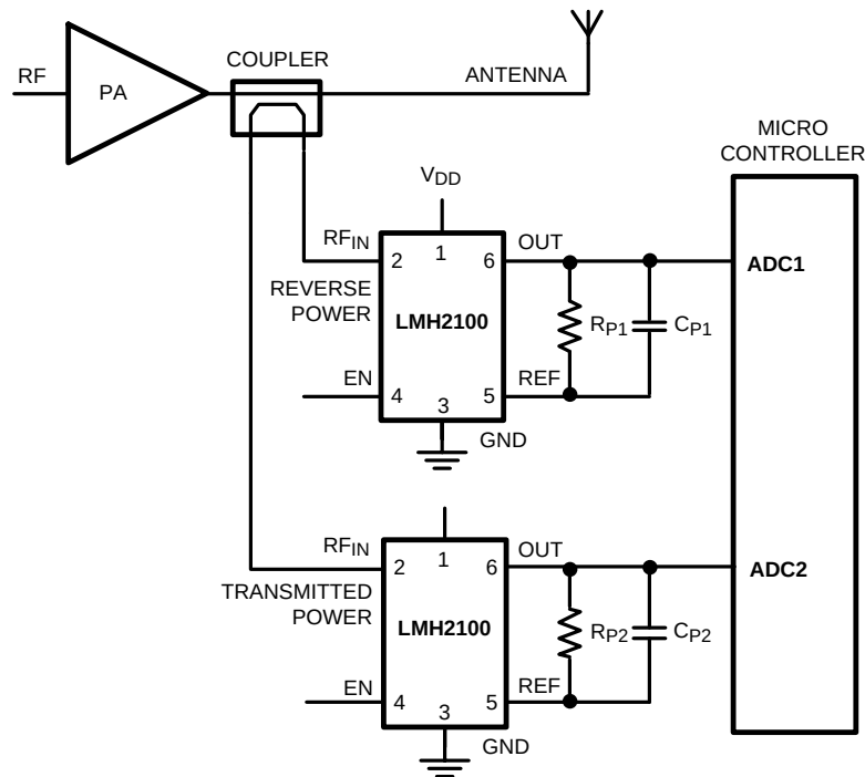
Figure 88. VSWR Application
