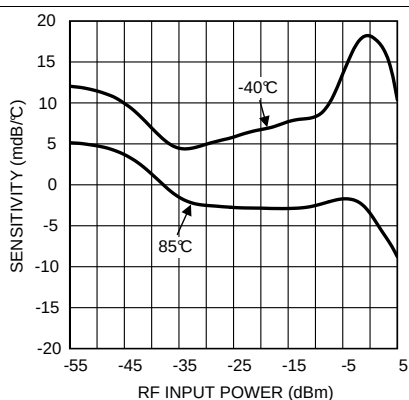
Figure 49. Mean Temperature Sensitivity vs RF Input Power at 1855 MHz
