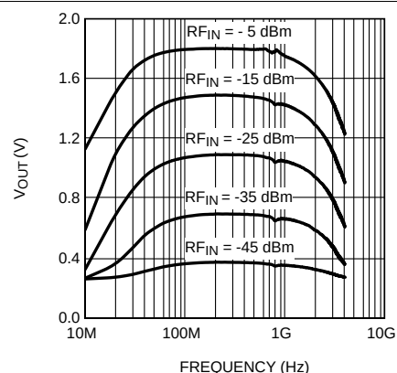
Figure 87. Output Voltage vs Frequency
