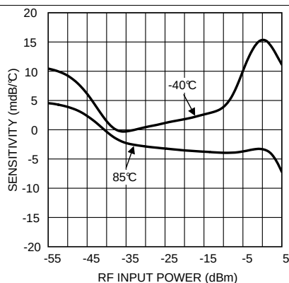
Figure 47. Mean Temperature Sensitivity vs RF Input Power at 50 MHz
