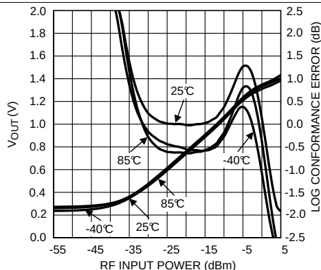
Figure 11. Mean Output Voltage and Log Conformance Error vs RF Input Power at 4000 MHz
