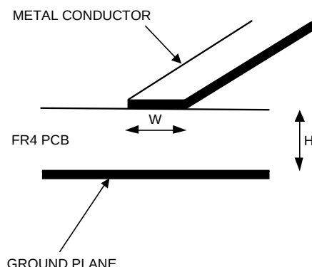
Figure 89. Microstrip Configuration
