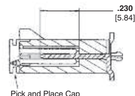
Section K-K
