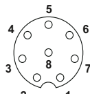
Socket, 8-pos.
