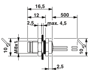
M8 flush-type plug, M8 fastening thread
