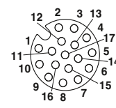
Socket, 17-pos.
