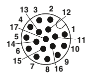
Plug, 17-pos.
