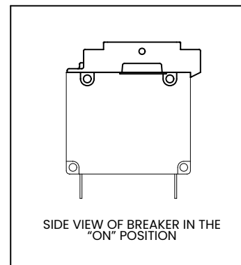
PUSH-TO-RESET ACTUATOR
