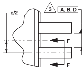
DETAIL G
