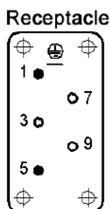
View from cable side
