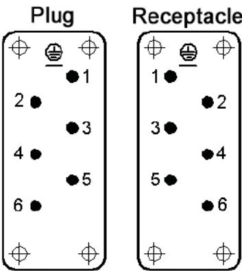
View from cable side
