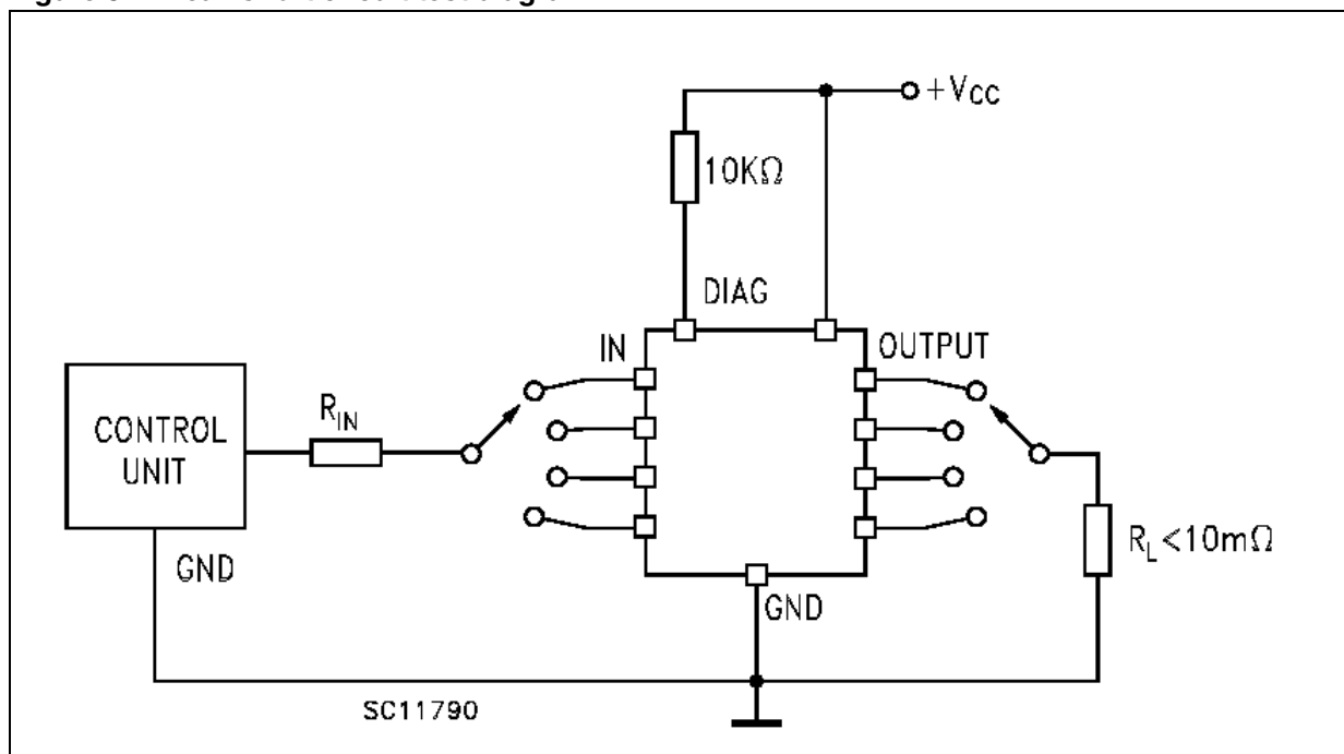
Figure 5. Peak short circuit test diagram
