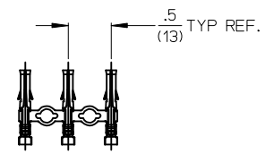
SECT. "C-C"
