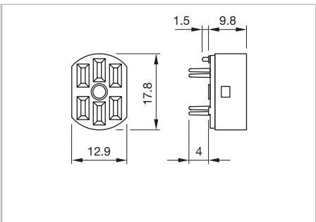
Dimensions [mm] for Part No. 31-942
