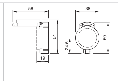
Dimensions [mm] for Part No. 704.928.28, 704.928.38
