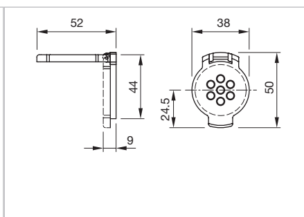
Dimensions [mm] for Part No. 704.928.18
