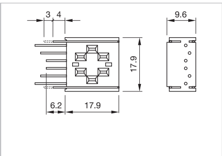
Dimensions [mm] for Part No. 31-941
