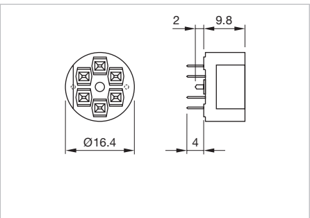
Dimensions [mm] for Part No. 31-940
