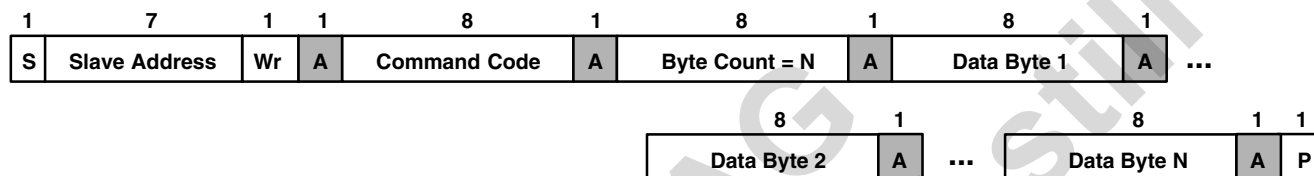
Figure 20. SMBus Block Write or I²C Write Protocols
