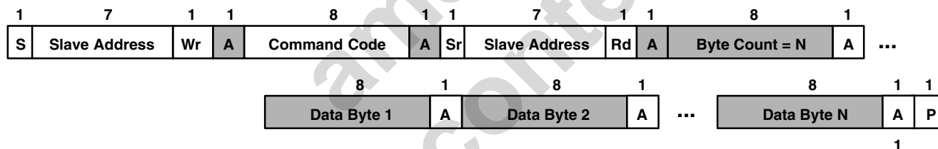
Figure 21. SMBus Block Read or I²C Read (Combined Format) Protocols
