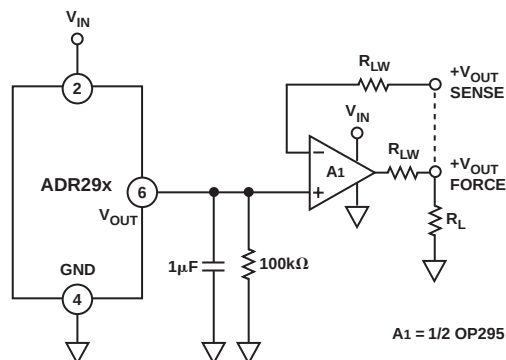
Figure 35. Advantage of Kelvin Connection
