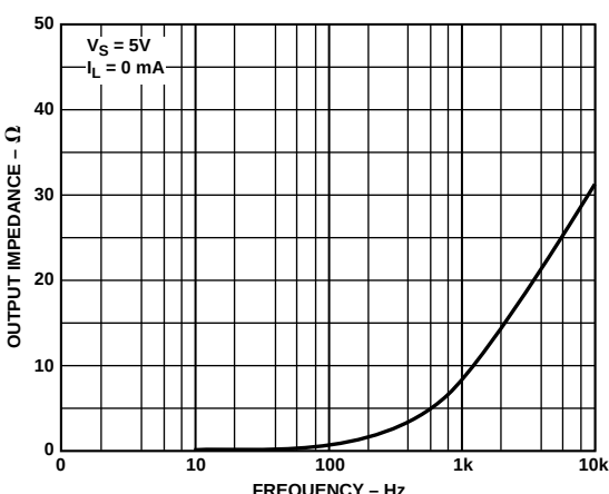
Figure 23. ADR291 Output Impedance vs. Frequency
