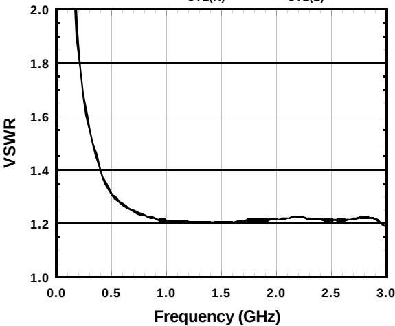
VSWR(P1) vs. Frequency
