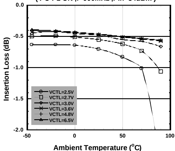
Insertion Loss vs. Ambient Temperature
