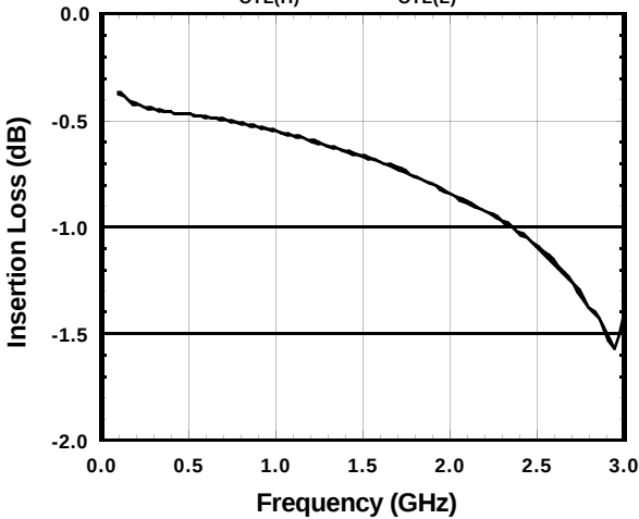
PC-P4 Insertion Loss vs. Frequency
