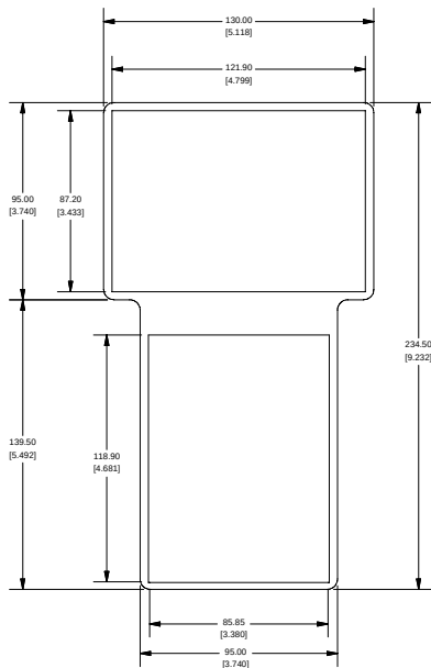
FRONT VIEW OF LID
