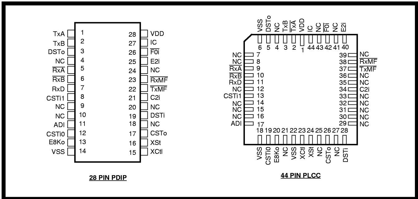
Figure 2 - Pin Connections
