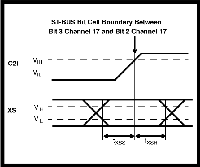
Figure 23 - XS Timing
