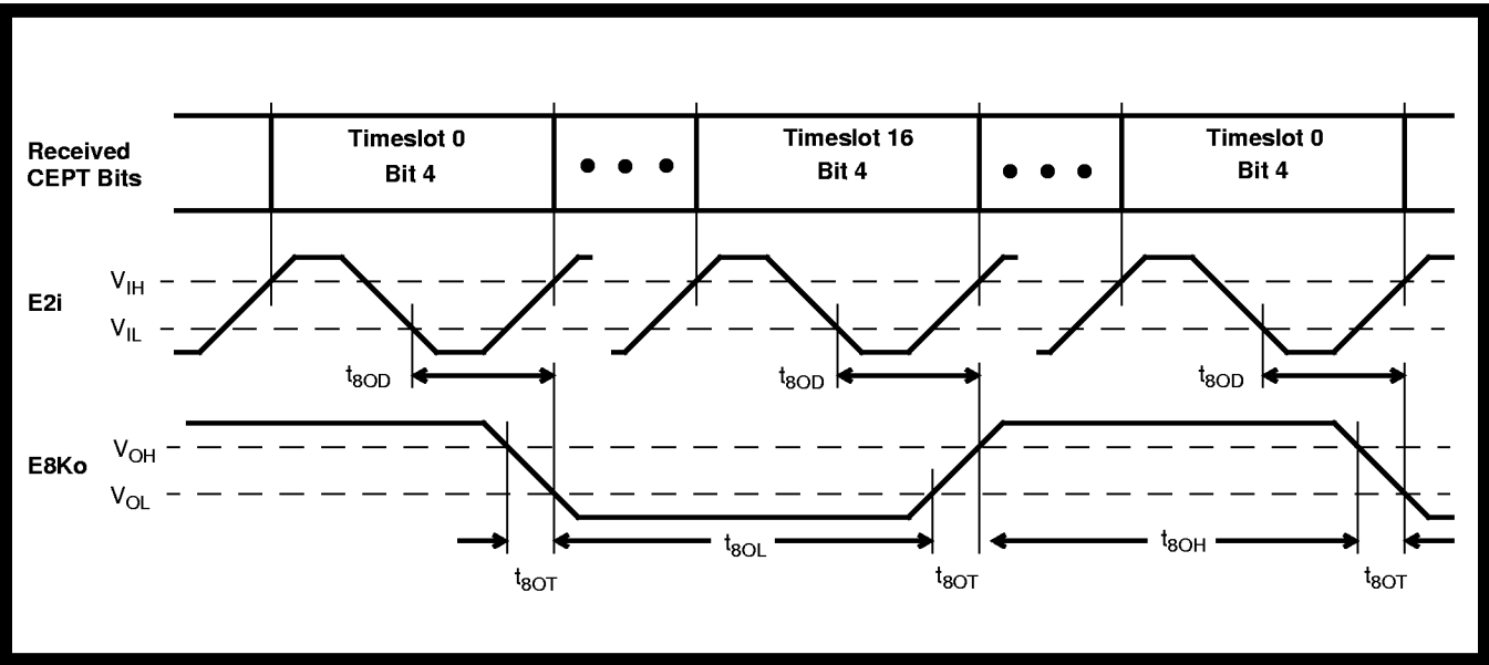
Figure 24 - E8Ko Timing
