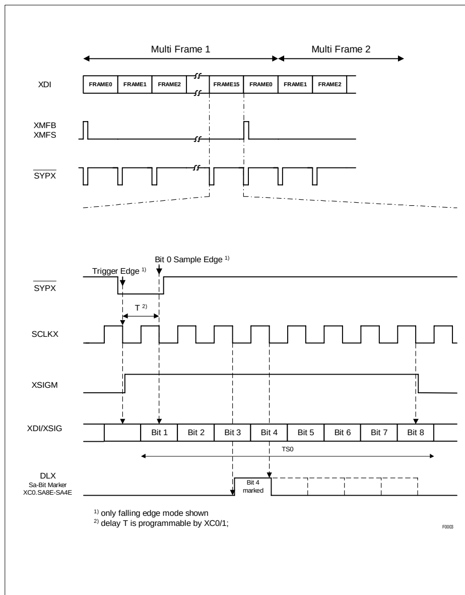
Figure 33 Transmit System Interface Clocking: 2.048 MHz (E1)
