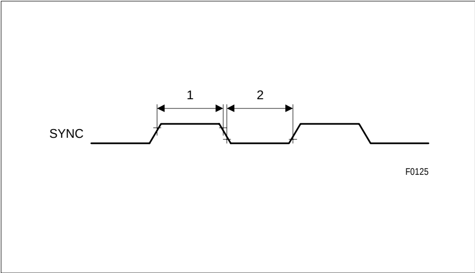
Figure 102 SYNC Timing
