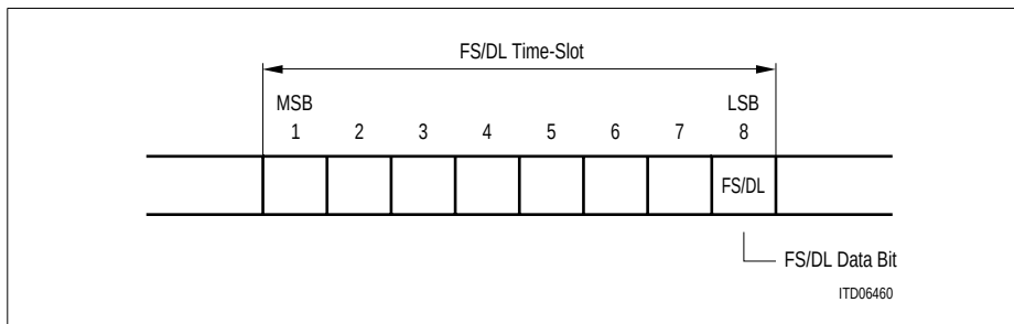
Figure 69 Transmit FS/DL Bits on XDI (T1/J1)
