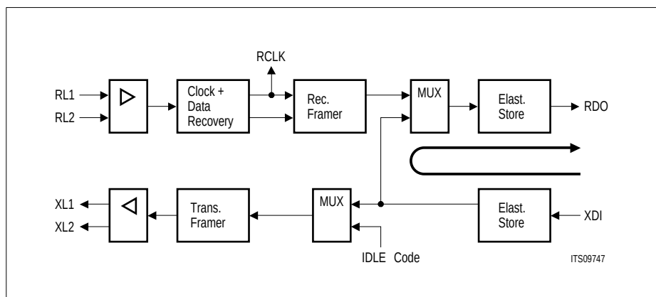
Figure 40 Single Channel Loop-Back (E1)
