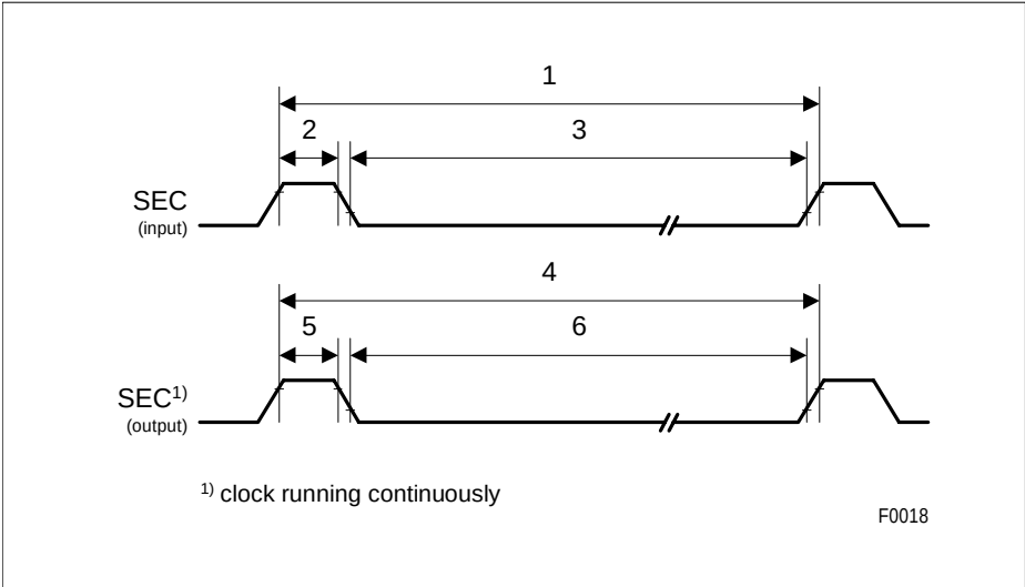
Figure 100 SEC Timing
