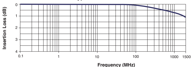
CX2038 - Typical Insertion Loss @ 25°C
