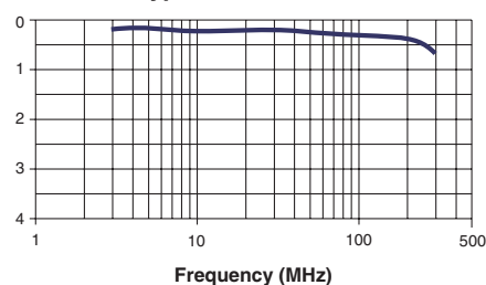
CX2045 - Typical Insertion Loss @ 25°C
