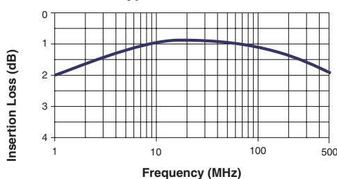
CX2040 - Typical Insertion Loss @ 25°C
