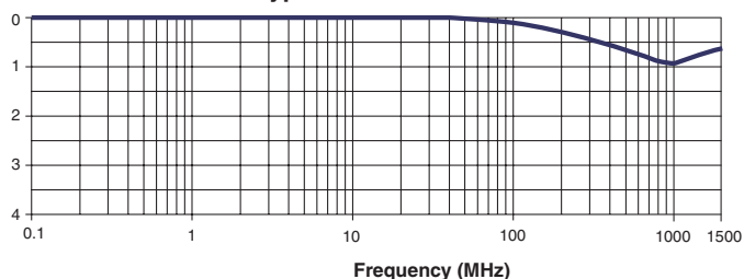
CX2039 - Typical Insertion Loss @ 25°C
