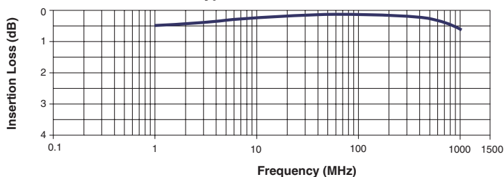
CX2043 - Typical Insertion Loss @ 25°C
