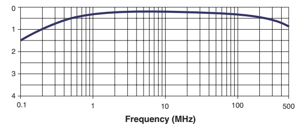
CX2047 - Typical Insertion Loss @ 25°C
