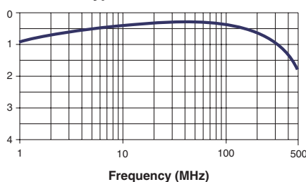
CX2044 - Typical Insertion Loss @ 25°C
