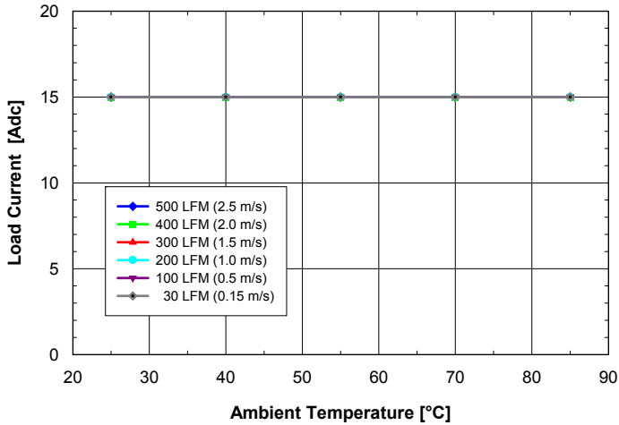
Fig. 1.5V.1: Available load current vs. ambient air temperature and airflow rates for SQ24T15015 converter with B height pins mounted vertically with V_{in} = 24V , air flowing from pin 3 to pin 1 and maximum FET temperature \leq 120^{\circ}C .
