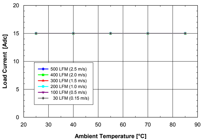
Fig. 1.0V.3: Available load current vs. ambient temperature and airflow rates for SQ24S15010 converter mounted vertically with V_{in} = 24V , air flowing from pin 3 to pin 1 and maximum FET temperature \leq 120^{\circ}C .
