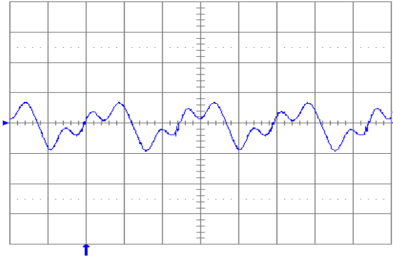
Fig. 2.0V.13: Output voltage ripple (20 mV/div.) at full rated load current into a resistive load with C_o = 10\ \mu\text{F} tantalum + 1\ \mu\text{F} ceramic and V_{in} = 24\ \text{V} . Time scale: 1\ \mu\text{s}/\text{div} .
