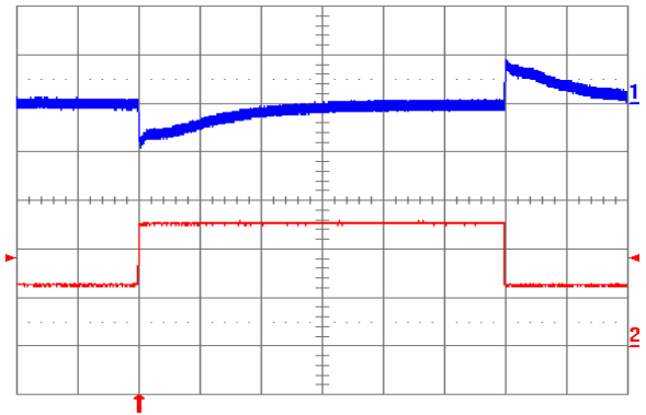
Fig. 5.0V.12: Output voltage response to load current step-change (2.5A – 5A – 2.5A) at V_{in} = 24V . Top trace: output voltage (100 mV/div.). Bottom trace: load current (2 A/div.). Current slew rate: 5 A/ \mu s . C_o = 450 \mu F tantalum + 1 \mu F ceramic. Time scale: 0.2 ms/div.
