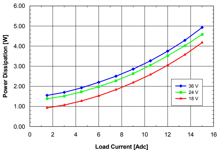
Fig. 1.5V.7: Power dissipation vs. load current and input voltage for SQ24T/S15015 converter mounted vertically with air flowing from pin 3 to pin 1 at a rate of 300 LFM (1.5 m/s) and T_a = 25^\circ\text{C} .
