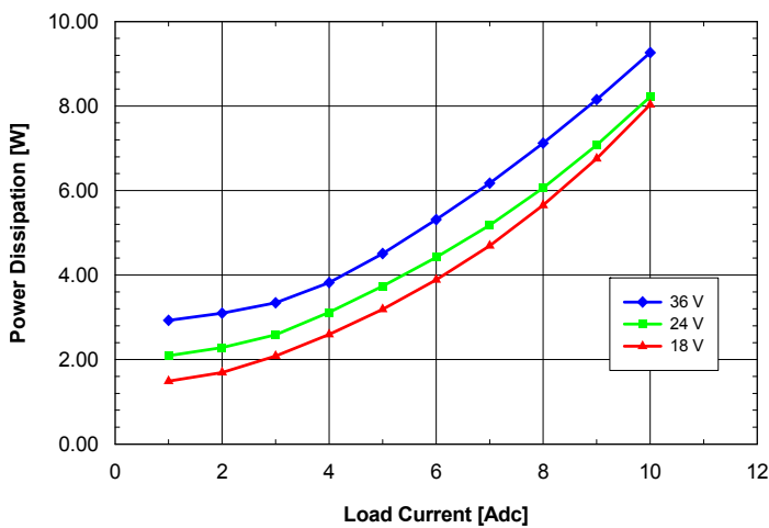
Fig. 5.0V.7: Power dissipation vs. load current and input voltage for SQ24T/S10050 converter mounted vertically with air flowing from pin 3 to pin 1 at a rate of 300 LFM (1.5 m/s) and T_a = 25^\circ\text{C} .
