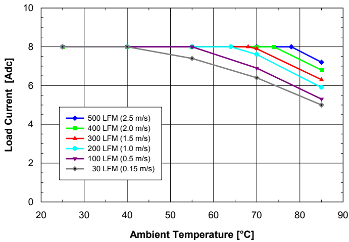
Fig. 6.0V.1: Available load current vs. ambient air temperature and airflow rates for SQ24T08060 converter with B height pins mounted vertically with V_{in} = 24V , air flowing from pin 3 to pin 1 and maximum FET temperature \leq 120^{\circ}C .
