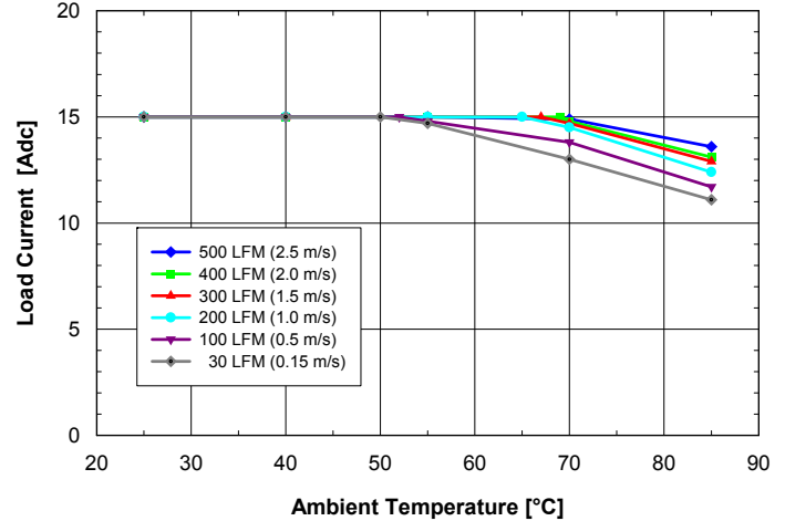
Fig. 2.5V.4: Available load current vs. ambient temperature and airflow rates for SQ24S15025 converter mounted horizontally with V_{in} = 24V , air flowing from pin 3 to pin 1 and maximum FET temperature \leq 120^{\circ}C .
