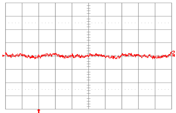
Fig. 6.0V.16: Input reflected ripple current, i_s (10 mA/div.), measured through 10\ \mu\text{H} at the source at full rated load current and V_{in} = 24\ \text{V} . Refer to Fig. 6.0V.14 for test setup. Time scale: 1\ \mu\text{s}/\text{div} .
