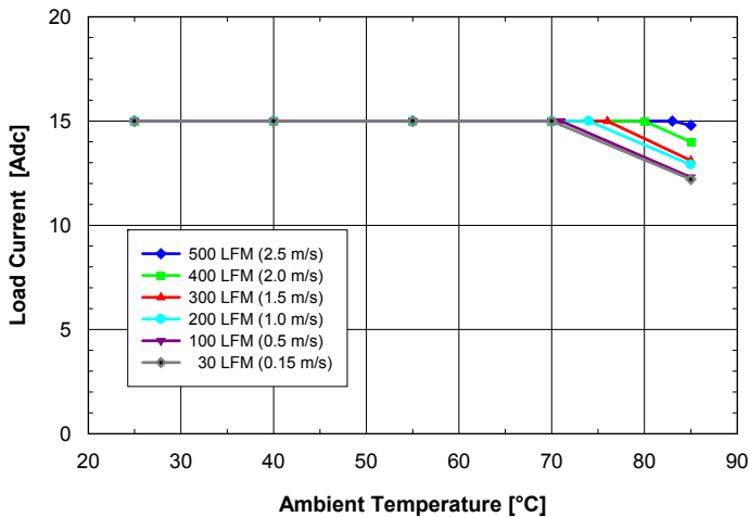
Fig. 2.5V.1: Available load current vs. ambient air temperature and airflow rates for SQ24T15025 converter with B height pins mounted vertically with V_{in} = 24V , air flowing from pin 3 to pin 1 and maximum FET temperature \leq 120^{\circ}C .
