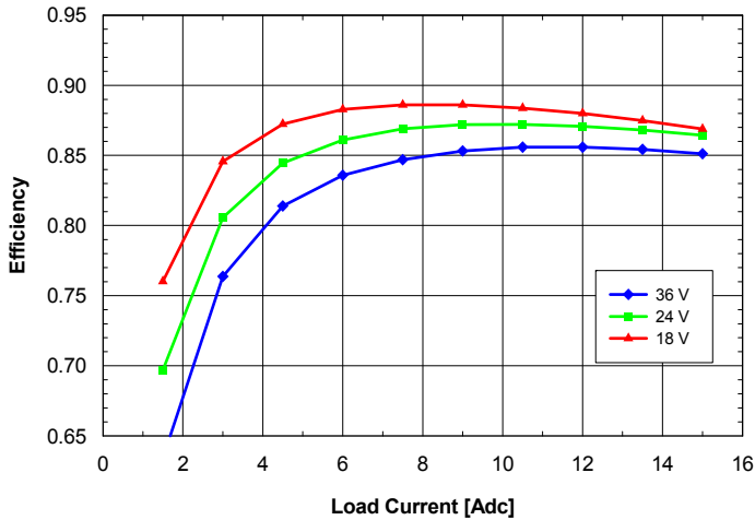
Fig. 2.5V.5: Efficiency vs. load current and input voltage for SQ24T/S15025 converter mounted vertically with air flowing from pin 3 to pin 1 at a rate of 300 LFM (1.5 m/s) and T_a = 25^\circ\text{C} .
