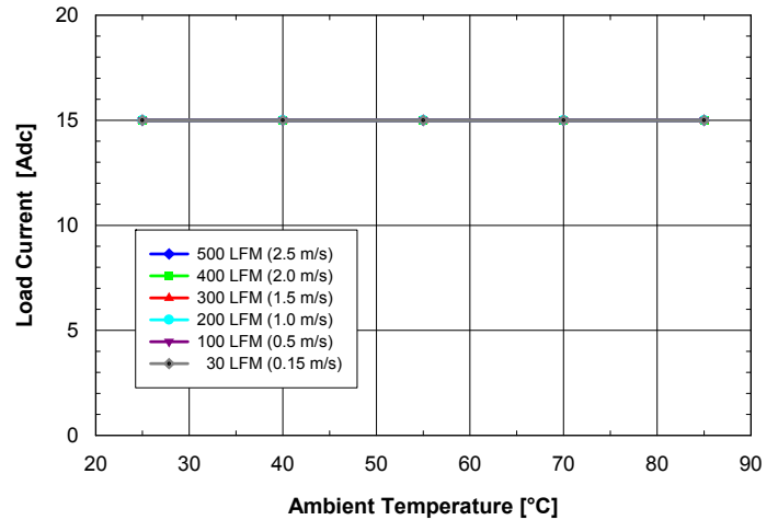
Fig. 1.5V.4: Available load current vs. ambient temperature and airflow rates for SQ24S15015 converter mounted horizontally with V_{in} = 24V , air flowing from pin 3 to pin 1 and maximum FET temperature \leq 120^{\circ}C .
