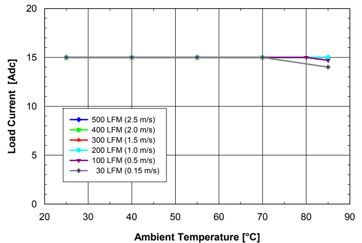
Fig. 2.0V.4: Available load current vs. ambient temperature and airflow rates for SQ24S15020 converter mounted horizontally with V_{in} = 24V , air flowing from pin 3 to pin 1 and maximum FET temperature \leq 120^{\circ}C .
