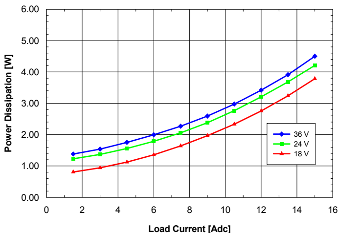
Fig. 1.2V.7: Power dissipation vs. load current and input voltage for SQ24T/S15012 converter mounted vertically with air flowing from pin 3 to pin 1 at a rate of 300 LFM (1.5 m/s) and T_a = 25^\circ\text{C} .
