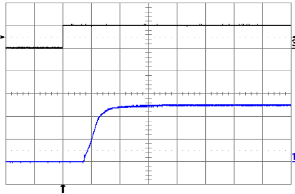
Fig. 5.0V.9: Turn-on transient at full rated load current (resistive) with no output capacitor at V_{in} = 24V , triggered via ON/OFF pin. Top trace: ON/OFF signal (5 V/div.). Bottom trace: output voltage (2 V/div.). Time scale: 2 ms/div.
