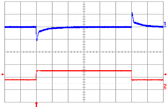
Fig. 1.0V.12: Output voltage response to load current step-change (3.75 A – 7.5 A – 3.75 A) at V_{in} = 24V . Top trace: output voltage (100 mV/div.). Bottom trace: load current (5 A/div.). Current slew rate: 5 A/µs. C_o = 450 \mu F tantalum + 1 µF ceramic. Time scale: 0.2 ms/div.
