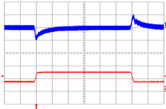
Fig. 1.5V.11: Output voltage response to load current step-change (3.75 A – 7.5 A – 3.75 A) at V_{in} = 24V . Top trace: output voltage (100 mV/div.). Bottom trace: load current (5 A/div.). Current slew rate: 0.1 A/ \mu s . C_o = 1 \mu F ceramic. Time scale: 0.2 ms/div.
