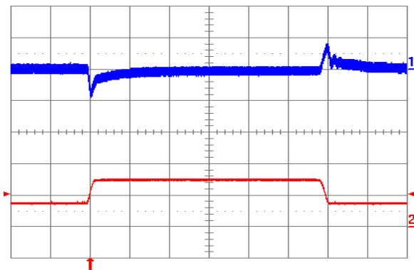
Fig. 1.8V.11: Output voltage response to load current step-change (3.75A – 7.5A – 3.75A) at V_{in} = 24V . Top trace: output voltage (100 mV/div.). Bottom trace: load current (5 A/div.). Current slew rate: 0.1 A/µs. C_o = 1 \mu F ceramic. Time scale: 0.2 ms/div.
