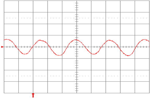
Fig. 5.0V.15: Input reflected ripple current, i_c (100 mA/div.), measured at input terminals at full rated load current and V_{in} = 24 \text{ V} . Refer to Fig. 5.0V.14 for test setup. Time scale: 1 \mu\text{s}/\text{div} .
