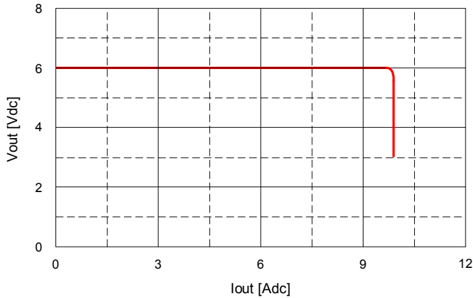
Fig. 6.0V.17: Output voltage vs. load current showing current limit point and converter shutdown point. Input voltage has almost no effect on current limit characteristic.
