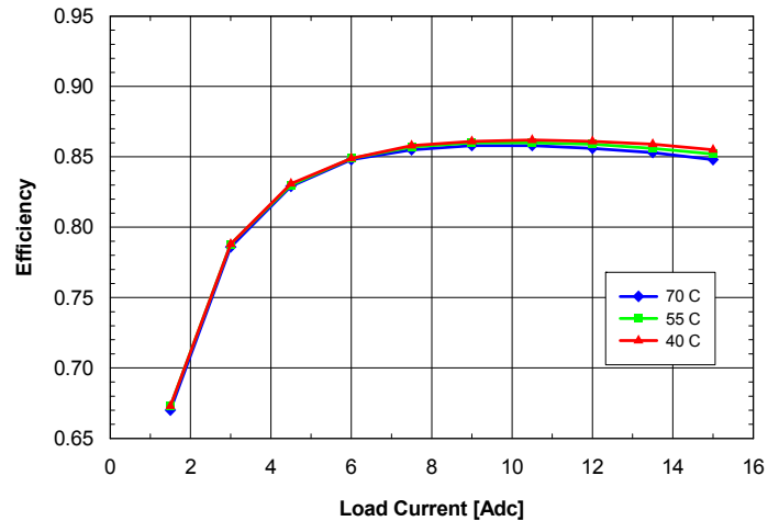
Fig. 2.0V.6: Efficiency vs. load current and ambient temperature for SQ24T/S15020 converter mounted vertically with V_{in} = 24\text{V} and air flowing from pin 3 to pin 1 at a rate of 200 LFM (1.0 m/s).
