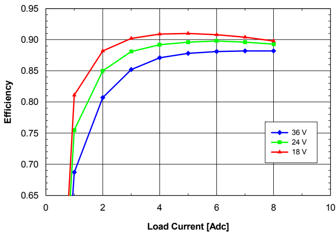
Fig. 6.0V.5: Efficiency vs. load current and input voltage for SQ24T/S08060 converter mounted vertically with air flowing from pin 3 to pin 1 at a rate of 300 LFM (1.5 m/s) and T_a = 25^\circ\text{C} .
