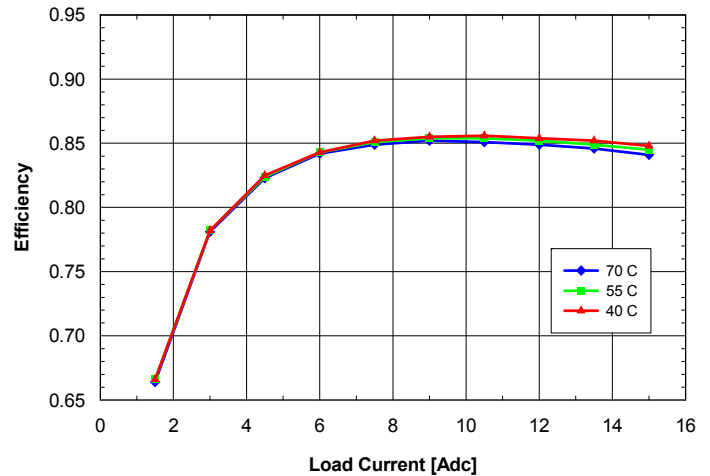
Fig. 1.8V.6: Efficiency vs. load current and ambient temperature for SQ24T/S15018 converter mounted vertically with V_{in} = 24\text{V} and air flowing from pin 3 to pin 1 at a rate of 200 LFM (1.0 m/s).
