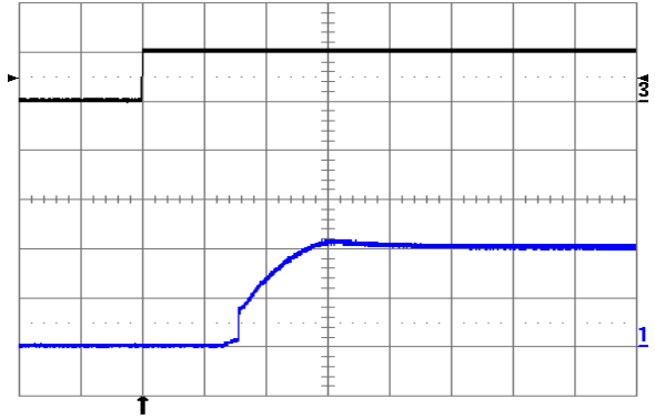
Fig. 1.0V.10: Turn-on transient at full rated load current (resistive) plus 10,000µF at V_{in} = 24V , triggered via ON/OFF pin. Top trace: ON/OFF signal (5 V/div.). Bottom trace: output voltage (0.5 V/div.). Time scale: 1 ms/div.
