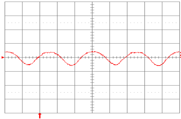
Fig. 1.5V.15: Input reflected ripple current, i_c (100 mA/div.), measured at input terminals at full rated load current and V_{in} = 24 \text{ V} . Refer to Fig. 1.5V.14 for test setup. Time scale: 1 \mu\text{s}/\text{div} .
