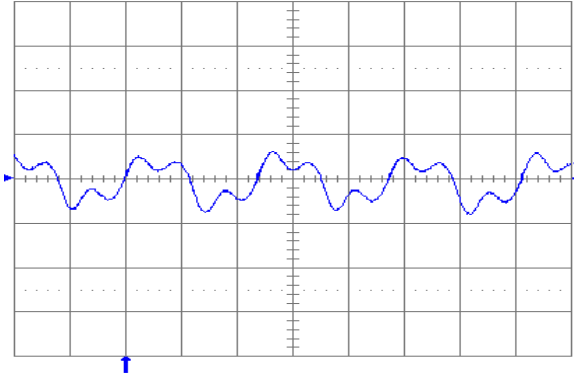
Fig. 2.5V.13: Output voltage ripple (20 mV/div.) at full rated load current into a resistive load with C_o = 10\ \mu\text{F} tantalum + 1\ \mu\text{F} ceramic and V_{in} = 24\ \text{V} . Time scale: 1\ \mu\text{s}/\text{div} .
