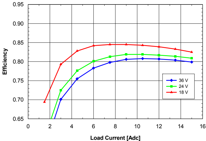
Fig. 1.2V.5: Efficiency vs. load current and input voltage for SQ24T/S15012 converter mounted vertically with air flowing from pin 3 to pin 1 at a rate of 300 LFM (1.5 m/s) and T_a = 25^\circ\text{C} .
