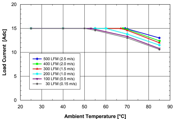
Fig. 2.5V.3: Available load current vs. ambient temperature and airflow rates for SQ24S15025 converter mounted vertically with V_{in} = 24V , air flowing from pin 3 to pin 1 and maximum FET temperature \leq 120^{\circ}C .
