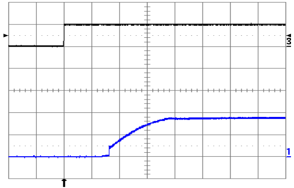
Fig. 1.8V.10: Turn-on transient at full rated load current (resistive) plus 10,000µF at V_{in} = 24V , triggered via ON/OFF pin. Top trace: ON/OFF signal (5 V/div.). Bottom trace: output voltage (1 V/div.). Time scale: 1 ms/div.
