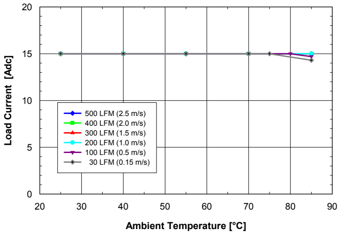
Fig. 1.8V.1: Available load current vs. ambient air temperature and airflow rates for SQ24T15018 converter with B height pins mounted vertically with V_{in} = 24V , air flowing from pin 3 to pin 1 and maximum FET temperature \leq 120^{\circ}C .
