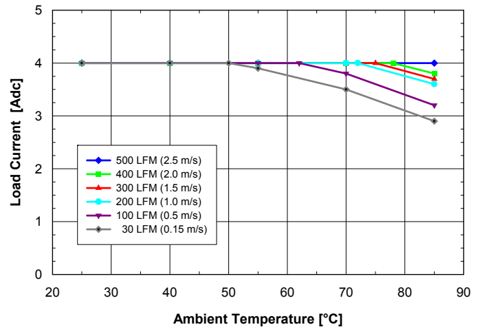
Fig. 12V.4: Available load current vs. ambient temperature and airflow rates for SQ24S04120 converter mounted horizontally with V_{in} = 24V , air flowing from pin 3 to pin 1 and maximum FET temperature \leq 120^{\circ}C .
