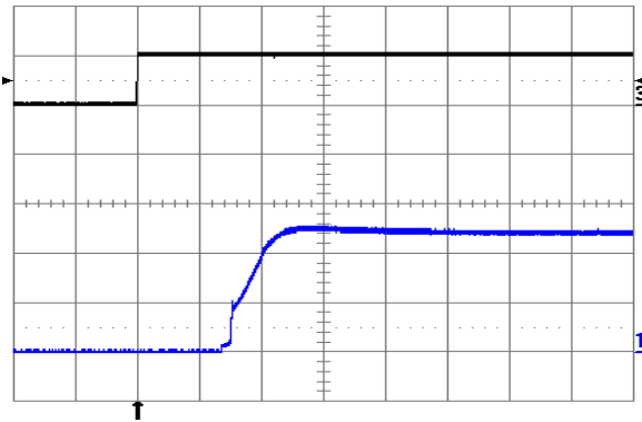
Fig. 1.2V.9: Turn-on transient at full rated load current (resistive) with no output capacitor at V_{in} = 24V , triggered via ON/OFF pin. Top trace: ON/OFF signal (5 V/div.). Bottom trace: output voltage (0.5 V/div.). Time scale: 1 ms/div.
