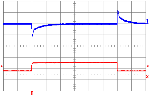
Fig. 1.5V.12: Output voltage response to load current step-change (3.75 A – 7.5 A – 3.75 A) at V_{in} = 24V . Top trace: output voltage (100 mV/div.). Bottom trace: load current (5 A/div.). Current slew rate: 5 A/ \mu s . C_o = 450 \mu F tantalum + 1 \mu F ceramic. Time scale: 0.2 ms/div.
