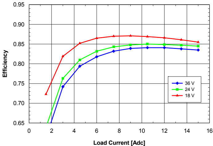
Fig. 1.8V.5: Efficiency vs. load current and input voltage for SQ24T/S15018 converter mounted vertically with air flowing from pin 3 to pin 1 at a rate of 300 LFM (1.5 m/s) and T_a = 25^\circ\text{C} .
