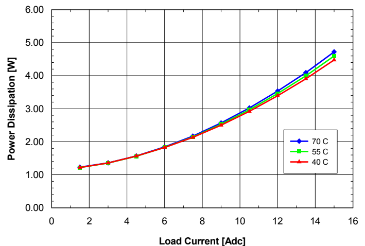
Fig. 1.5V.8: Power dissipation vs. load current and ambient temperature for SQ24T/S15015 converter mounted vertically with V_{in} = 24\text{V} and air flowing from pin 3 to pin 1 at a rate of 200 LFM (1.0 m/s).
