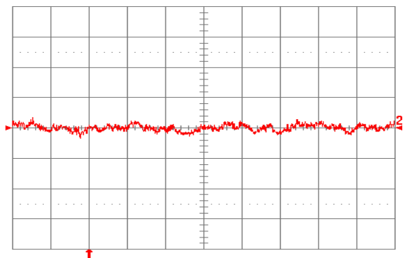
Fig. 2.0V.16: Input reflected ripple current, i_s (10 mA/div.), measured through 10\ \mu\text{H} at the source at full rated load current and V_{in} = 24\ \text{V} . Refer to Fig. 2.0V.14 for test setup. Time scale: 1\ \mu\text{s}/\text{div} .
