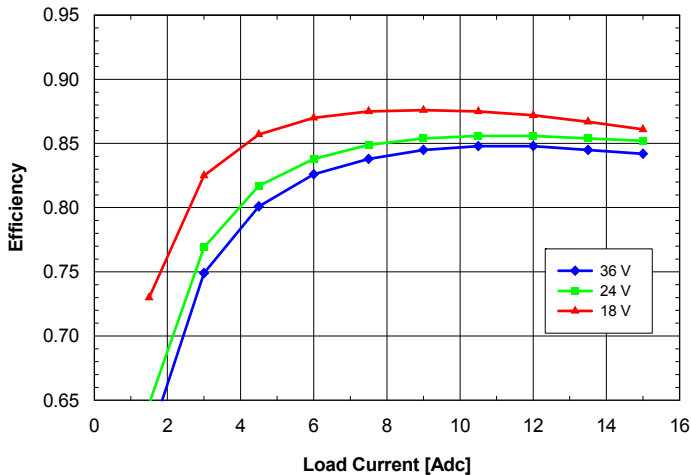
Fig. 2.0V.5: Efficiency vs. load current and input voltage for SQ24T/S15020 converter mounted vertically with air flowing from pin 3 to pin 1 at a rate of 300 LFM (1.5 m/s) and T_a = 25^\circ\text{C} .
