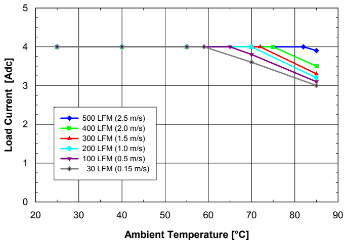
Fig. 12V.3: Available load current vs. ambient temperature and airflow rates for SQ24S04120 converter mounted vertically with V_{in} = 24V , air flowing from pin 3 to pin 1 and maximum FET temperature \leq 120^{\circ}C .
