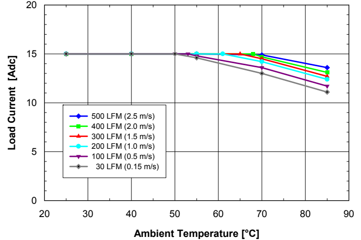
Fig. 3.3V.4: Available load current vs. ambient temperature and airflow rates for SQ24S15033 converter mounted horizontally with V_{in} = 24V , air flowing from pin 3 to pin 1 and maximum FET temperature \leq 120^{\circ}C .
