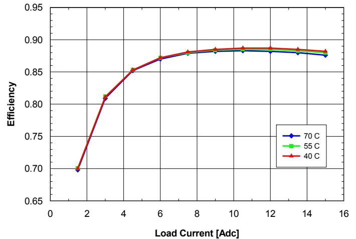
Fig. 3.3V.6: Efficiency vs. load current and ambient temperature for SQ24T/S15033 converter mounted vertically with V_{in} = 24\text{V} and air flowing from pin 3 to pin 1 at a rate of 200 LFM (1.0 m/s).
