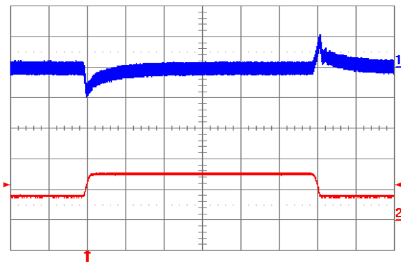
Fig. 2.5V.11: Output voltage response to load current step-change (3.75 A – 7.5 A – 3.75 A) at V_{in} = 24V . Top trace: output voltage (100 mV/div.). Bottom trace: load current (5 A/div.). Current slew rate: 0.1 A/ \mu s . C_o = 1 \mu F ceramic. Time scale: 0.2 ms/div.
