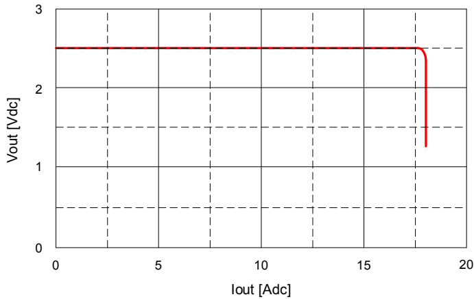
Fig. 2.5V.17: Output voltage vs. load current showing current limit point and converter shutdown point. Input voltage has almost no effect on current limit characteristic.
