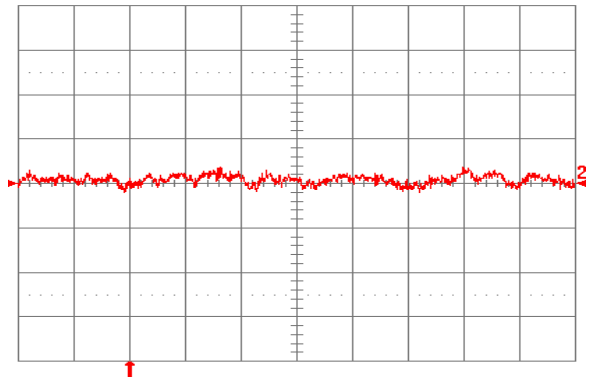
Fig. 1.0V.16: Input reflected ripple current, i_s (10 mA/div.), measured through 10\ \mu\text{H} at the source at full rated load current and V_{in} = 24\ \text{V} . Refer to Fig. 1.0V.14 for test setup. Time scale: 1\ \mu\text{s}/\text{div} .
