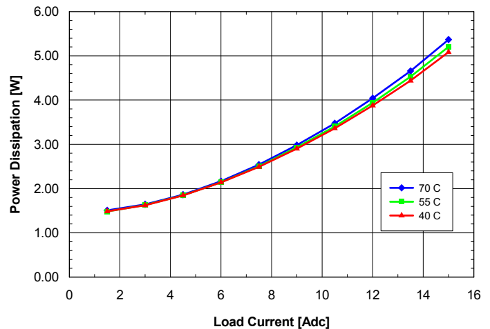
Fig. 2.0V.8: Power dissipation vs. load current and ambient temperature for SQ24T/S15020 converter mounted vertically with V_{in} = 24\text{V} and air flowing from pin 3 to pin 1 at a rate of 200 LFM (1.0 m/s).
