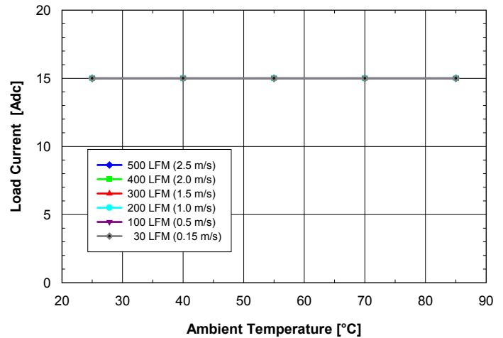
Fig. 1.2V.2: Available load current vs. ambient air temperature and airflow rates for SQ24T15012 converter with B height pins mounted horizontally with V_{in} = 24V , air flowing from pin 3 to pin 1 and maximum FET temperature \leq 120^{\circ}C .
