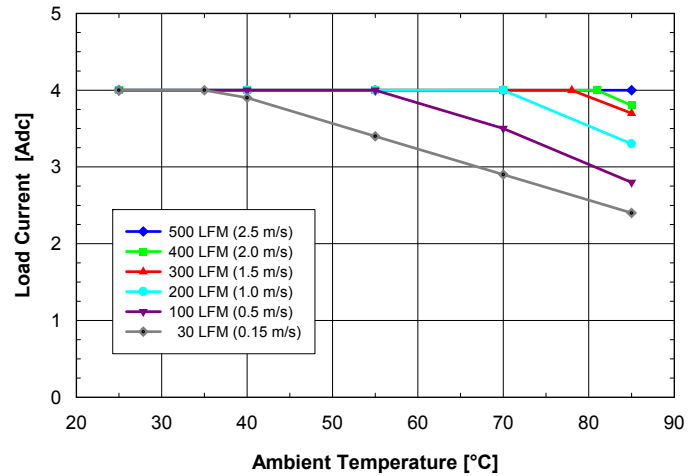
Fig. 12V.2: Available load current vs. ambient air temperature and airflow rates for SQ24T04120 converter with B height pins mounted horizontally with V_{in} = 24V , air flowing from pin 3 to pin 1 and maximum FET temperature \leq 120^{\circ}C .
