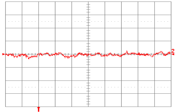
Fig. 3.3V.16: Input reflected ripple current, i_s (10 mA/div.), measured through 10\ \mu\text{H} at the source at full rated load current and V_{in} = 24\ \text{V} . Refer to Fig. 3.3V.14 for test setup. Time scale: 1\ \mu\text{s}/\text{div} .
