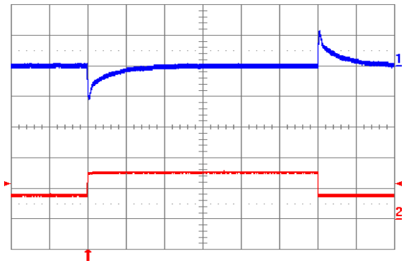
Fig. 2.5V.12: Output voltage response to load current step-change (3.75 A – 7.5 A – 3.75 A) at V_{in} = 24V . Top trace: output voltage (100 mV/div.). Bottom trace: load current (5 A/div.). Current slew rate: 5 A/ \mu s . C_o = 450 \mu F tantalum + 1 \mu F ceramic. Time scale: 0.2 ms/div.
