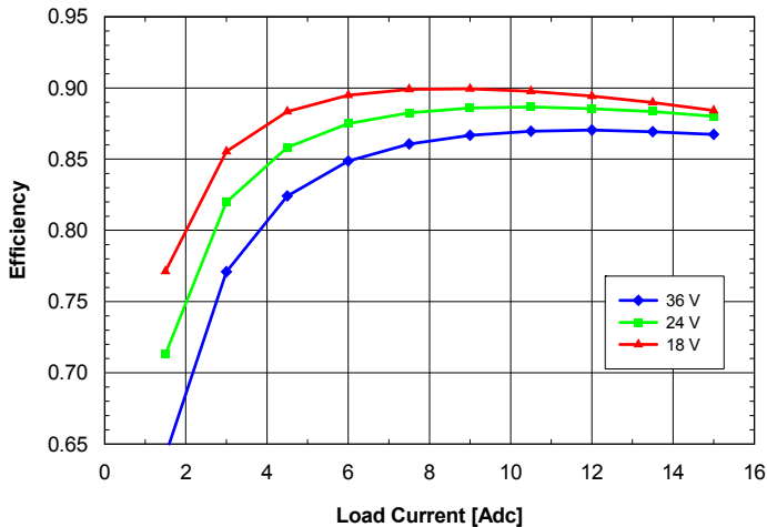
Fig. 3.3V.5: Efficiency vs. load current and input voltage for SQ24T/S15033 converter mounted vertically with air flowing from pin 3 to pin 1 at a rate of 300 LFM (1.5 m/s) and T_a = 25^\circ\text{C} .
