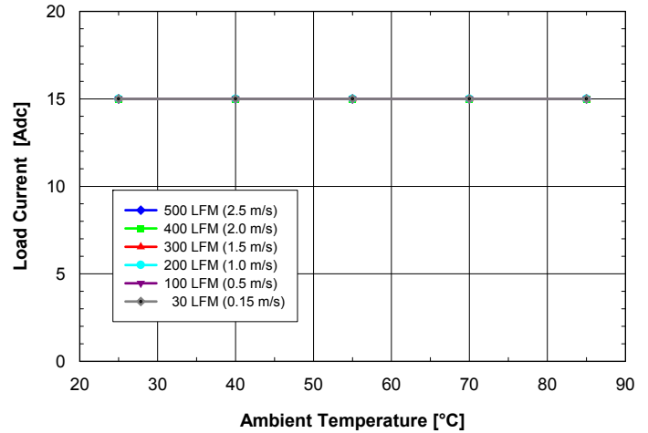
Fig. 1.5V.2: Available load current vs. ambient air temperature and airflow rates for SQ24T15015 converter with B height pins mounted horizontally with V_{in} = 24V , air flowing from pin 3 to pin 1 and maximum FET temperature \leq 120^{\circ}C .
