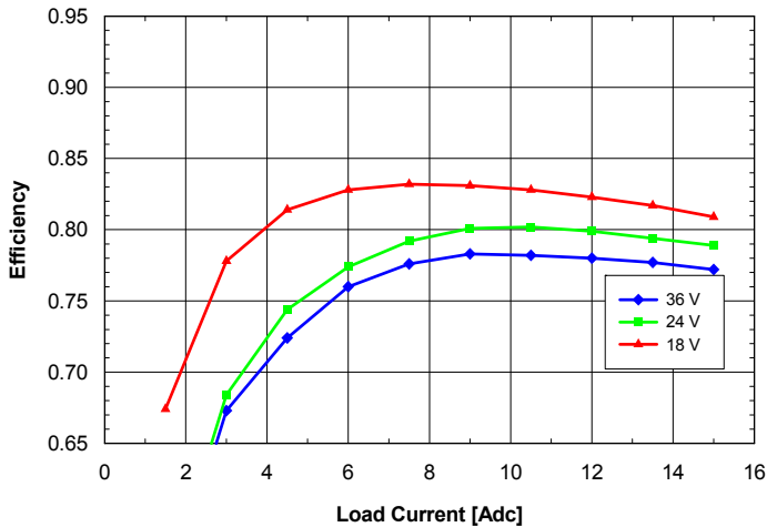
Fig. 1.0V.5: Efficiency vs. load current and input voltage for SQ24T/S15010 converter mounted vertically with air flowing from pin 3 to pin 1 at a rate of 300 LFM (1.5 m/s) and T_a = 25^\circ\text{C} .
