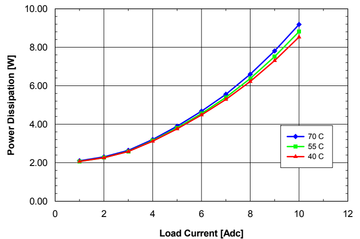
Fig. 5.0V.8: Power dissipation vs. load current and ambient temperature for SQ24T/S10050 converter mounted vertically with V_{in} = 24\text{V} and air flowing from pin 3 to pin 1 at a rate of 200 LFM (1.0 m/s).
