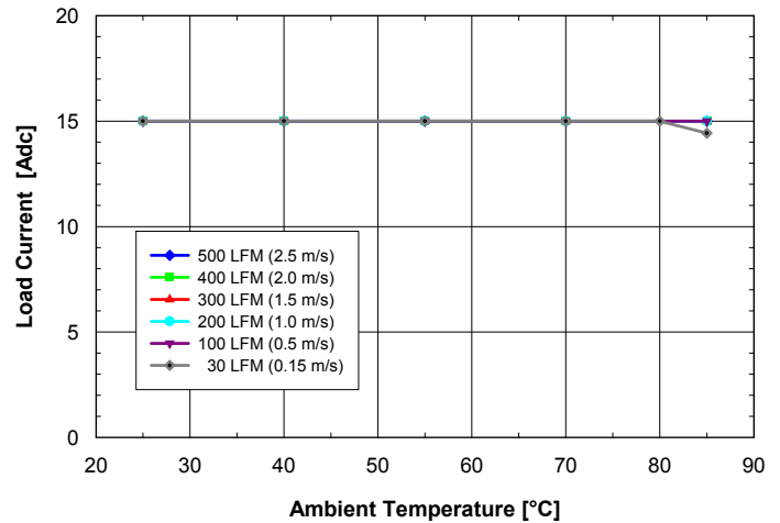
Fig. 1.8V.2: Available load current vs. ambient air temperature and airflow rates for SQ24T15018 converter with B height pins mounted horizontally with V_{in} = 24V , air flowing from pin 3 to pin 1 and maximum FET temperature \leq 120^{\circ}C .
