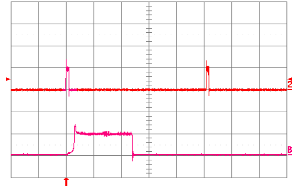
Fig. 2.5V.18: Load current (top trace, 20 A/div., 20 ms/div.) into a 10 mΩ short circuit during restart, at V_{in} = 24V . Bottom trace (20 A/div., 1 ms/div.) is an expansion of the on-time portion of the top trace.
