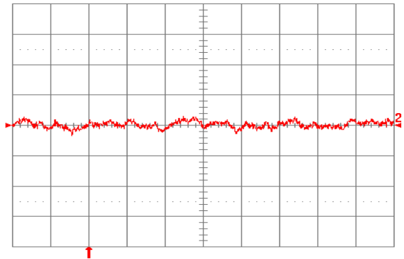
Fig. 5.0V.16: Input reflected ripple current, i_s (10 mA/div.), measured through 10 \mu\text{H} at the source at full rated load current and V_{in} = 24 \text{ V} . Refer to Fig. 5.0V.14 for test setup. Time scale: 1 \mu\text{s}/\text{div} .
