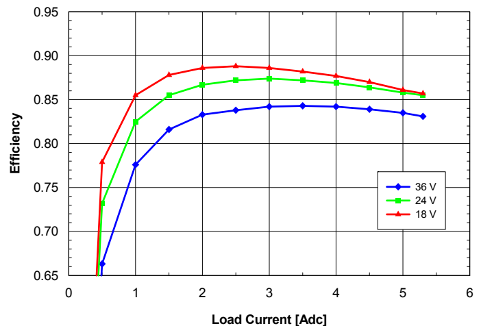
Fig. 8.0V.2: Efficiency vs. load current and input voltage for SQ24T/S05080 converter mounted vertically with air flowing from pin 3 to pin 1 at a rate of 300 LFM (1.5 m/s) and T_A = 25^\circ\text{C} .
