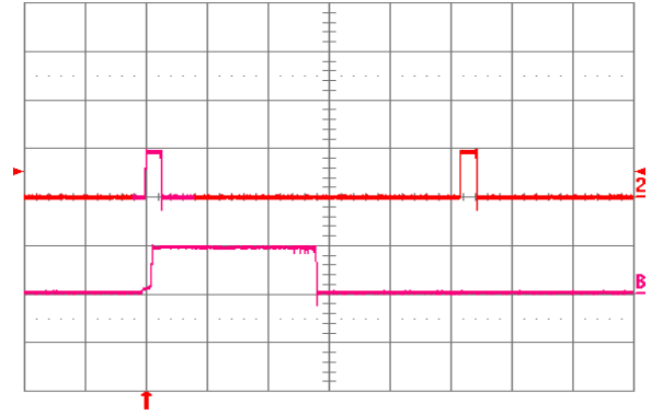
Fig. 1.5V.18: Load current (top trace, 20 A/div., 20 ms/div.) into a 10 mΩ short circuit during restart, at Vin = 24V. Bottom trace (20 A/div., 2 ms/div.) is an expansion of the on-time portion of the top trace.
