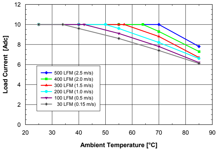
Fig. 5.0V.1: Available load current vs. ambient air temperature and airflow rates for SQ24T10050 converter with B height pins mounted vertically with V_{in} = 24V , air flowing from pin 3 to pin 1 and maximum FET temperature \leq 120^{\circ}C .
