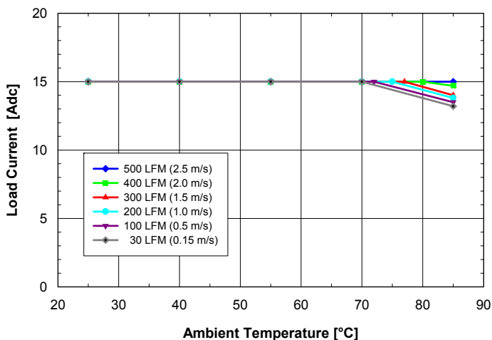
Fig. 2.0V.3: Available load current vs. ambient temperature and airflow rates for SQ24S15020 converter mounted vertically with V_{in} = 24V , air flowing from pin 3 to pin 1 and maximum FET temperature \leq 120^{\circ}C .
