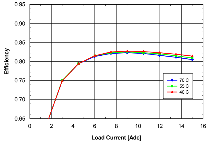
Fig. 1.2V.6: Efficiency vs. load current and ambient temperature for SQ24T/S15012 converter mounted vertically with V_{in} = 24\text{V} and air flowing from pin 3 to pin 1 at a rate of 200 LFM (1.0 m/s).
