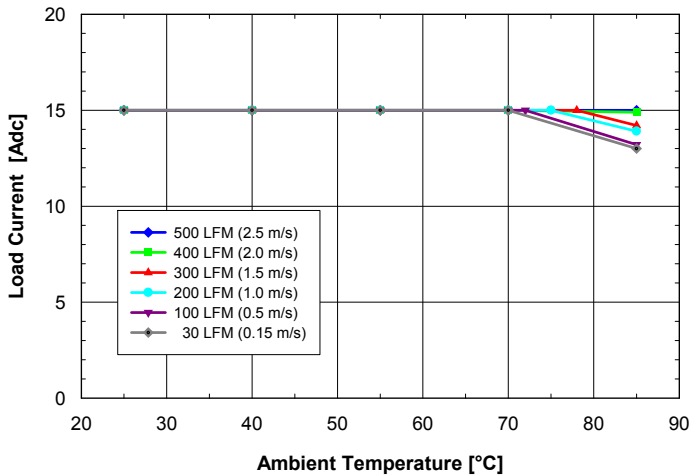
Fig. 2.0V.1: Available load current vs. ambient air temperature and airflow rates for SQ24T15020 converter with B height pins mounted vertically with V_{in} = 24V , air flowing from pin 3 to pin 1 and maximum FET temperature \leq 120^{\circ}C .
