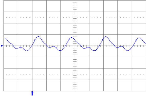
Fig. 3.3V.13: Output voltage ripple (20 mV/div.) at full rated load current into a resistive load with C_o = 10\ \mu\text{F} tantalum + 1\ \mu\text{F} ceramic and V_{in} = 24\ \text{V} . Time scale: 1\ \mu\text{s}/\text{div} .
