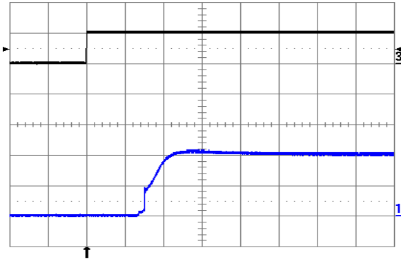
Fig. 1.0V.9: Turn-on transient at full rated load current (resistive) with no output capacitor at V_{in} = 24V , triggered via ON/OFF pin. Top trace: ON/OFF signal (5 V/div.). Bottom trace: output voltage (0.5 V/div.). Time scale: 1 ms/div.
