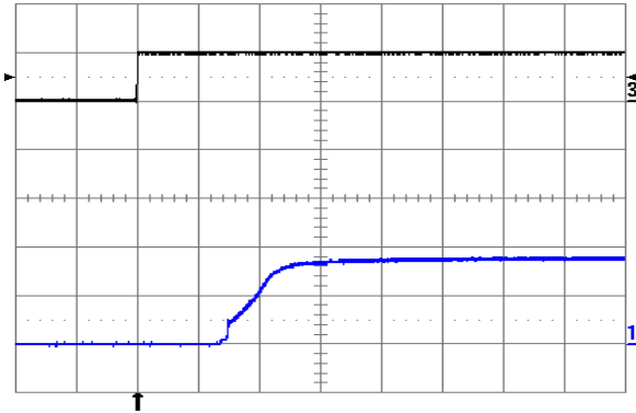
Fig. 1.8V.9: Turn-on transient at full rated load current (resistive) with no output capacitor at V_{in} = 24V , triggered via ON/OFF pin. Top trace: ON/OFF signal (5 V/div.). Bottom trace: output voltage (1 V/div.). Time scale: 1 ms/div.
