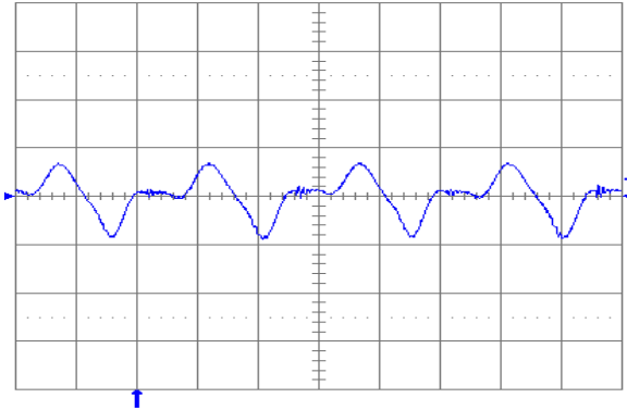
Fig. 1.5V.13: Output voltage ripple (20 mV/div.) at full rated load current into a resistive load with C_o = 10 \mu\text{F} tantalum + 1\mu\text{F} ceramic and V_{in} = 24 \text{ V} . Time scale: 1 \mu\text{s}/\text{div} .
