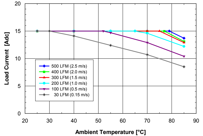
Fig. 3.3V.2: Available load current vs. ambient air temperature and airflow rates for SQ24T15033 converter with B height pins mounted horizontally with V_{in} = 24V , air flowing from pin 3 to pin 1 and maximum FET temperature \leq 120^{\circ}C .
