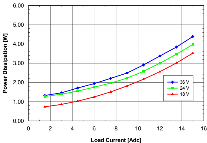
Fig. 1.0V.7: Power dissipation vs. load current and input voltage for SQ24T/S15010 converter mounted vertically with air flowing from pin 3 to pin 1 at a rate of 300 LFM (1.5 m/s) and T_a = 25^\circ\text{C} .
