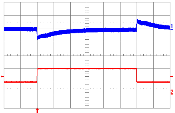
Fig. 6.0V.12: Output voltage response to load current step-change (2A – 4A – 2A) at V_{in} = 24V . Top trace: output voltage (100mV/div.). Bottom trace: load current (2A/div.). Current slew rate: 5 A/µs. C_o = 450 \mu F tantalum + 1 µF ceramic. Time scale: 0.2 ms/div.
