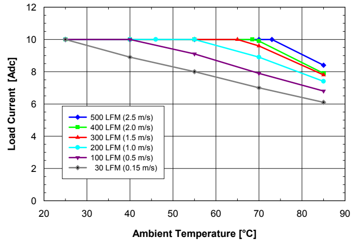
Fig. 5.0V.2: Available load current vs. ambient air temperature and airflow rates for SQ24T10050 converter with B height pins mounted horizontally with V_{in} = 24V , air flowing from pin 3 to pin 1 and maximum FET temperature \leq 120^{\circ}C .
