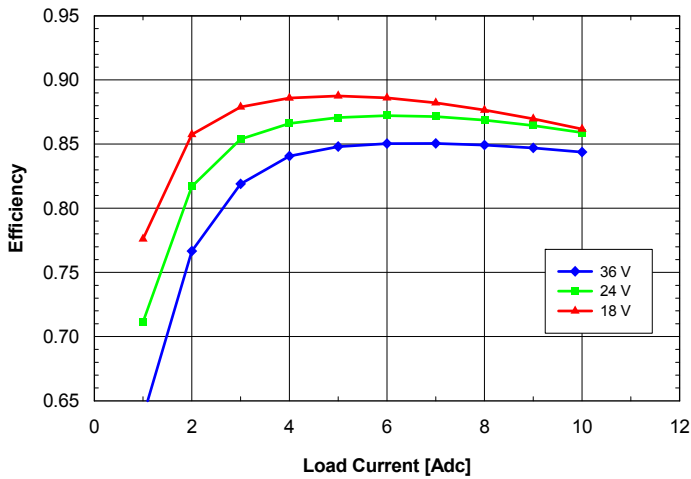
Fig. 5.0V.5: Efficiency vs. load current and input voltage for SQ24T/S10050 converter mounted vertically with air flowing from pin 3 to pin 1 at a rate of 300 LFM (1.5 m/s) and T_a = 25^\circ\text{C} .
