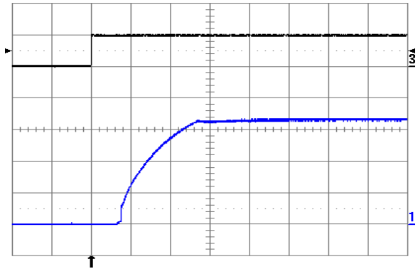
Fig. 3.3V.10: Turn-on transient at full rated load current (resistive) plus 10,000 \mu F at V_{in} = 24V , triggered via ON/OFF pin. Top trace: ON/OFF signal (5 V/div.). Bottom trace: output voltage (1 V/div.). Time scale: 2 ms/div.
