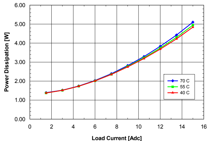
Fig. 1.8V.8: Power dissipation vs. load current and ambient temperature for SQ24T/S15018 converter mounted vertically with V_{in} = 24\text{V} and air flowing from pin 3 to pin 1 at a rate of 200 LFM (1.0 m/s).
