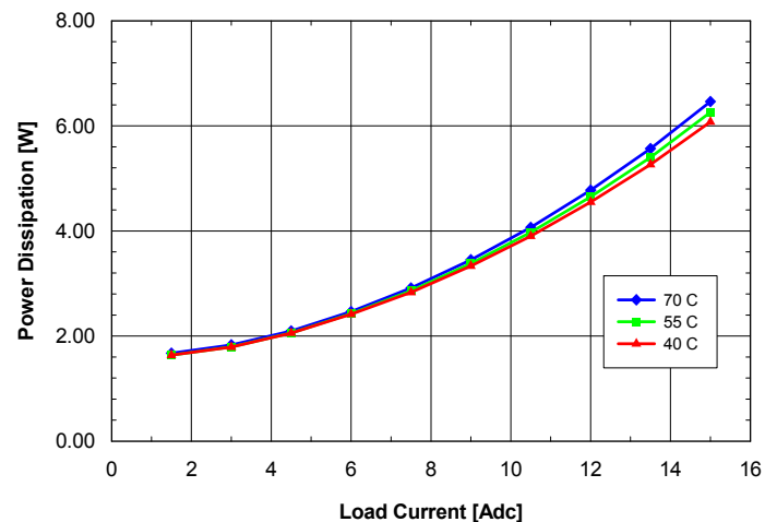
Fig. 2.5V.8: Power dissipation vs. load current and ambient temperature for SQ24T/S15025 converter mounted vertically with V_{in} = 24\text{V} and air flowing from pin 3 to pin 1 at a rate of 200 LFM (1.0 m/s).
