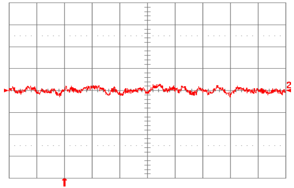
Fig. 1.5V.16: Input reflected ripple current, i_s (10 mA/div.), measured through 10 \mu\text{H} at the source at full rated load current and V_{in} = 24 \text{ V} . Refer to Fig. 1.5V.14 for test setup. Time scale: 1 \mu\text{s}/\text{div} .
