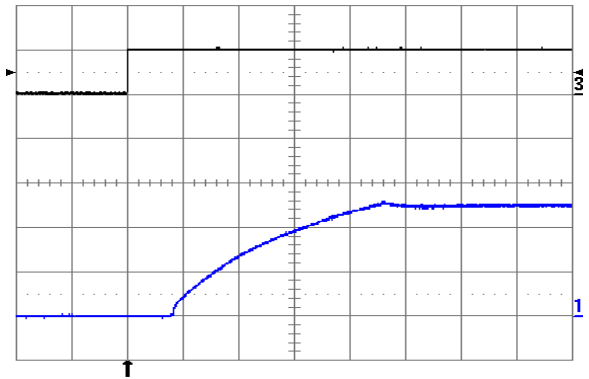
Fig. 5.0V.10: Turn-on transient at full rated load current (resistive) plus 10,000 \mu F at V_{in} = 24V , triggered via ON/OFF pin. Top trace: ON/OFF signal (5 V/div.). Bottom trace: output voltage (2 V/div.). Time scale: 2 ms/div.
