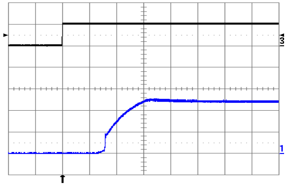
Fig. 1.2V.10: Turn-on transient at full rated load current (resistive) plus 10,000 \mu F at V_{in} = 24V , triggered via ON/OFF pin. Top trace: ON/OFF signal (5 V/div.). Bottom trace: output voltage (0.5 V/div.). Time scale: 1 ms/div.
