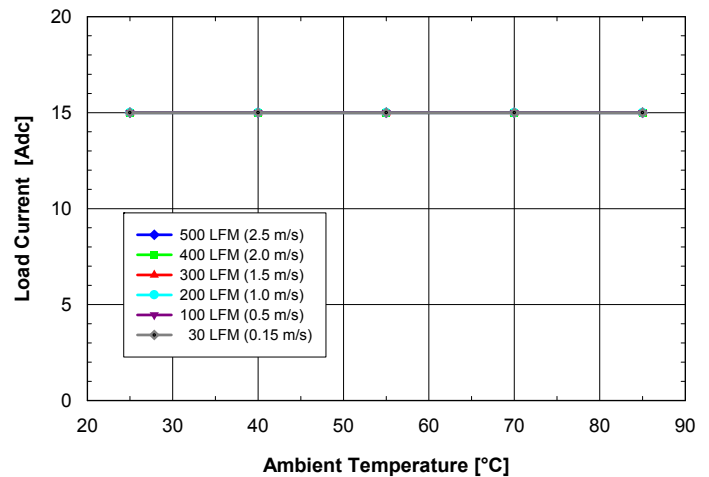
Fig. 1.0V.4: Available load current vs. ambient temperature and airflow rates for SQ24S15010 converter mounted horizontally with V_{in} = 24V , air flowing from pin 3 to pin 1 and maximum FET temperature \leq 120^{\circ}C .
