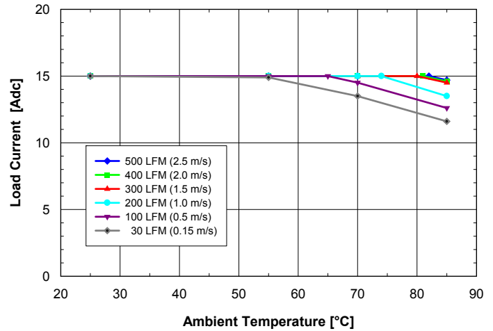
Fig. 2.5V.2: Available load current vs. ambient air temperature and airflow rates for SQ24T15025 converter with B height pins mounted horizontally with V_{in} = 24V , air flowing from pin 3 to pin 1 and maximum FET temperature \leq 120^{\circ}C .
