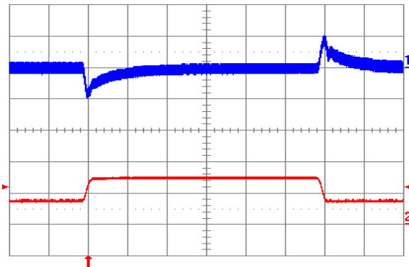
Fig. 1.2V.11: Output voltage response to load current step-change (3.75 A – 7.5 A – 3.75 A) at V_{in} = 24V . Top trace: output voltage (100 mV/div.). Bottom trace: load current (5 A/div.). Current slew rate: 0.1 A/ \mu s . C_o = 1 \mu F ceramic. Time scale: 0.2 ms/div.
