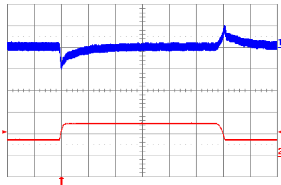
Fig. 3.3V.11: Output voltage response to load current step-change (3.75A – 7.5A – 3.75A) at V_{in} = 24V . Top trace: output voltage (100 mV/div.). Bottom trace: load current (5 A/div.). Current slew rate: 0.1 A/ \mu s . C_o = 1 \mu F ceramic. Time scale: 0.2 ms/div.
