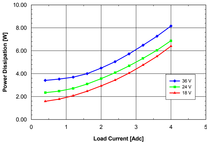
Fig. 12V.7: Power dissipation vs. load current and input voltage for SQ24T/S04120 converter mounted vertically with air flowing from pin 3 to pin 1 at a rate of 300 LFM (1.5 m/s) and T_a = 25^\circ\text{C} .
