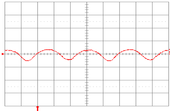
Fig. 1.2V.15: Input reflected ripple current, i_c (100 mA/div.), measured at input terminals at full rated load current and V_{in} = 24 \text{ V} . Refer to Fig. 1.2V.14 for test setup. Time scale: 1 \mu\text{s}/\text{div} .
