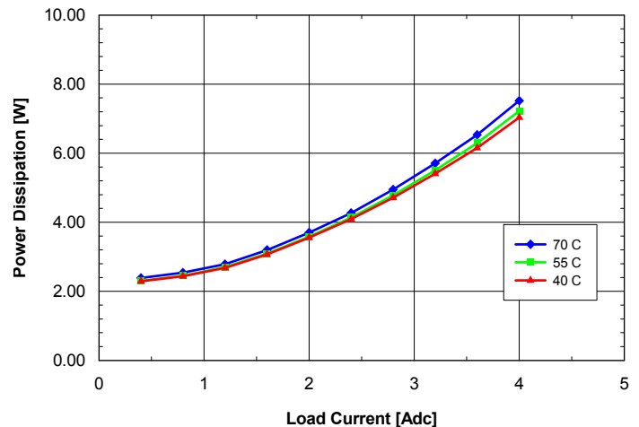
Fig. 12V.8: Power dissipation vs. load current and ambient temperature for SQ24T/S04120 converter mounted vertically with V_{in} = 24\text{V} and air flowing from pin 3 to pin 1 at a rate of 200 LFM (1.0 m/s).
