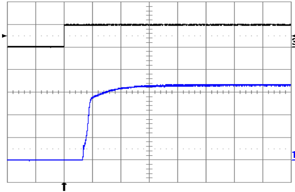
Fig. 3.3V.9: Turn-on transient at full rated load current (resistive) with no output capacitor at V_{in} = 24V , triggered via ON/OFF pin. Top trace: ON/OFF signal (5 V/div.). Bottom trace: output voltage (1 V/div.). Time scale: 2 ms/div.
