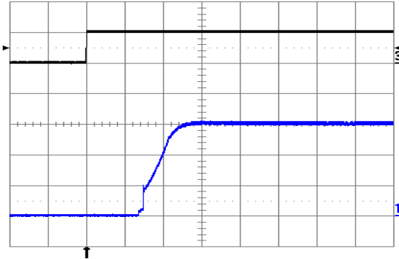
Fig. 1.5V.9: Turn-on transient at full rated load current (resistive) with no output capacitor at V_{in} = 24V , triggered via ON/OFF pin. Top trace: ON/OFF signal (5 V/div.). Bottom trace: output voltage (0.5 V/div.). Time scale: 1 ms/div.
