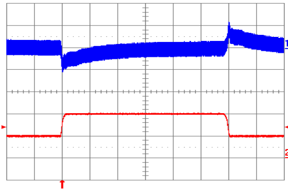
Fig. 6.0V.11: Output voltage response to load current step-change (2A – 4A – 2A) at V_{in} = 24V . Top trace: output voltage (100mV/div.). Bottom trace: load current (2A/div.). Current slew rate: 0.1 A/µs. C_o = 1 \mu F ceramic. Time scale: 0.2 ms/div.
