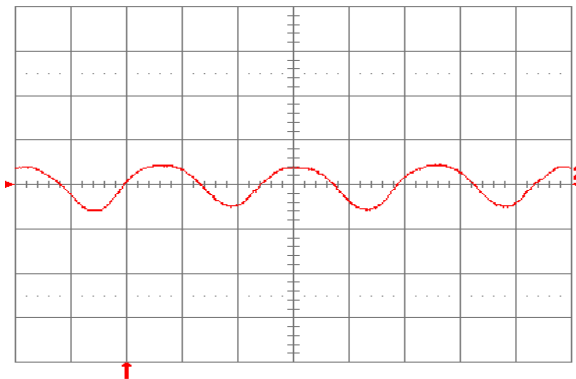
Fig. 1.8V.15: Input reflected ripple current, i_c (100 mA/div.), measured at input terminals at full rated load current and V_{in} = 24\ \text{V} . Refer to Fig. 1.8V.14 for test setup. Time scale: 1\ \mu\text{s}/\text{div} .
