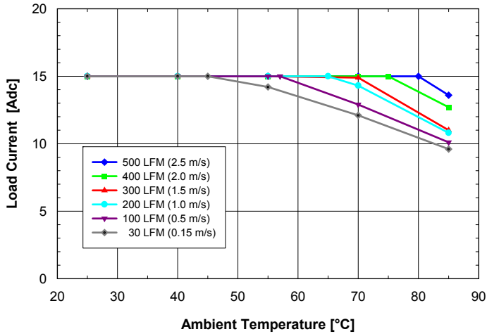
Fig. 3.3V.1: Available load current vs. ambient air temperature and airflow rates for SQ24T15033 converter with B height pins mounted vertically with V_{in} = 24V , air flowing from pin 3 to pin 1 and maximum FET temperature \leq 120^{\circ}C .
