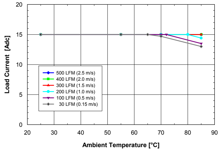
Fig. 2.0V.2: Available load current vs. ambient air temperature and airflow rates for SQ24T15020 converter with B height pins mounted horizontally with V_{in} = 24V , air flowing from pin 3 to pin 1 and maximum FET temperature \leq 120^{\circ}C .
