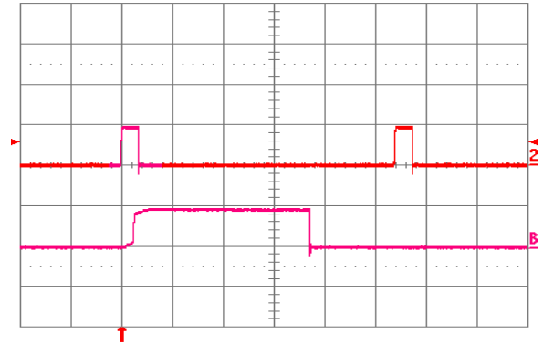
Fig. 1.0V.18: Load current (top trace, 20 A/div., 20 ms/div.) into a 10 mΩ short circuit during restart, at V_{in} = 24V . Bottom trace (20 A/div., 2 ms/div.) is an expansion of the on-time portion of the top trace.
