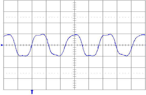
Fig. 5.0V.13: Output voltage ripple (20 mV/div.) at full rated load current into a resistive load with C_o = 10 \mu\text{F} tantalum + 1\mu\text{F} ceramic and V_{in} = 24 \text{ V} . Time scale: 1 \mu\text{s}/\text{div} .
