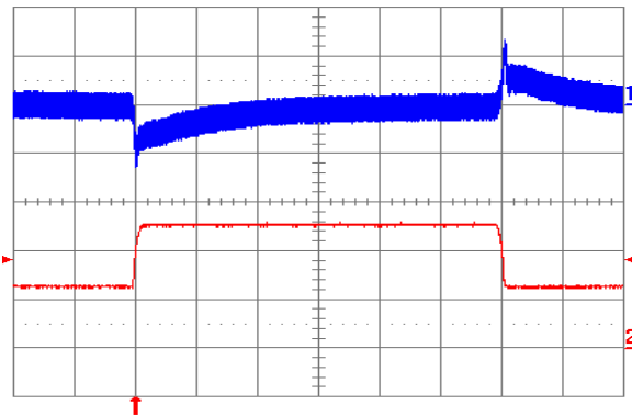
Fig. 5.0V.11: Output voltage response to load current step-change (2.5A – 5A – 2.5A) at V_{in} = 24V . Top trace: output voltage (100 mV/div.). Bottom trace: load current (2 A/div.). Current slew rate: 0.1 A/ \mu s . C_o = 1 \mu F ceramic. Time scale: 0.2 ms/div.
