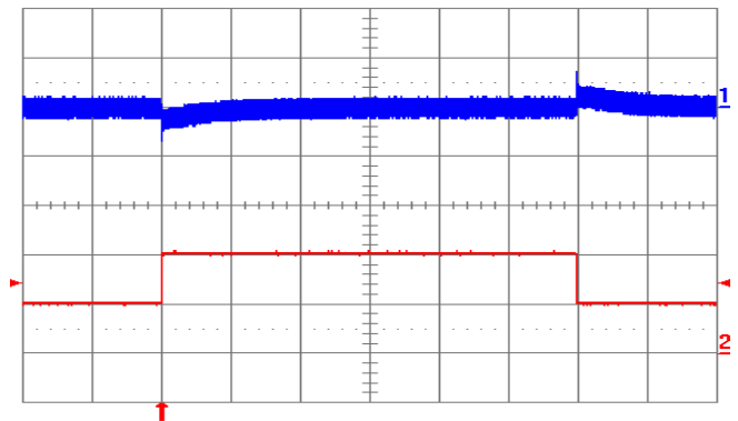
Fig. 12V.12: Output voltage response to load current step-change (1A – 2A – 1A) at V_{in} = 24V . Top trace: output voltage (200 mV/div.). Bottom trace: load current (1 A/div.). Current slew rate: 5 A/µs. C_o = 1 \mu F ceramic. Time scale: 0.5 ms/div.
