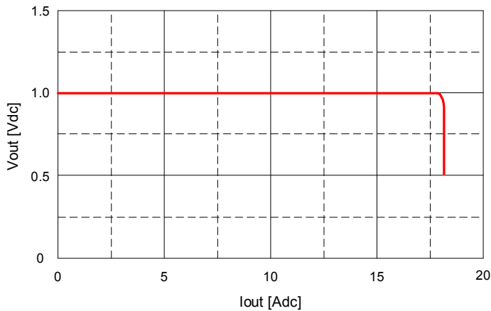
Fig. 1.0V.17: Output voltage vs. load current showing current limit point and converter shutdown point. Input voltage has almost no effect on current limit characteristic.
