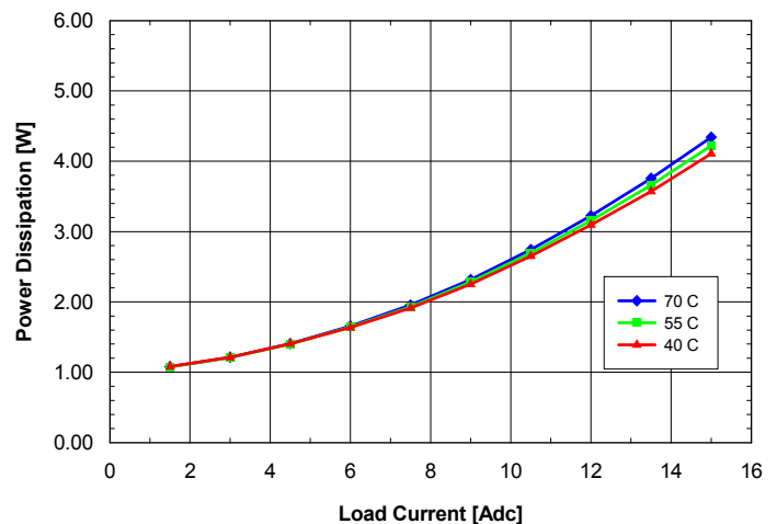
Fig. 1.2V.8: Power dissipation vs. load current and ambient temperature for SQ24T/S15012 converter mounted vertically with V_{in} = 24\text{V} and air flowing from pin 3 to pin 1 at a rate of 200 LFM (1.0 m/s).
