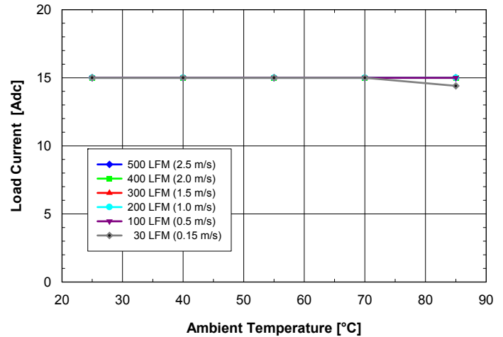
Fig. 1.8V.4: Available load current vs. ambient temperature and airflow rates for SQ24S15018 converter mounted horizontally with V_{in} = 24V , air flowing from pin 3 to pin 1 and maximum FET temperature \leq 120^{\circ}C .
