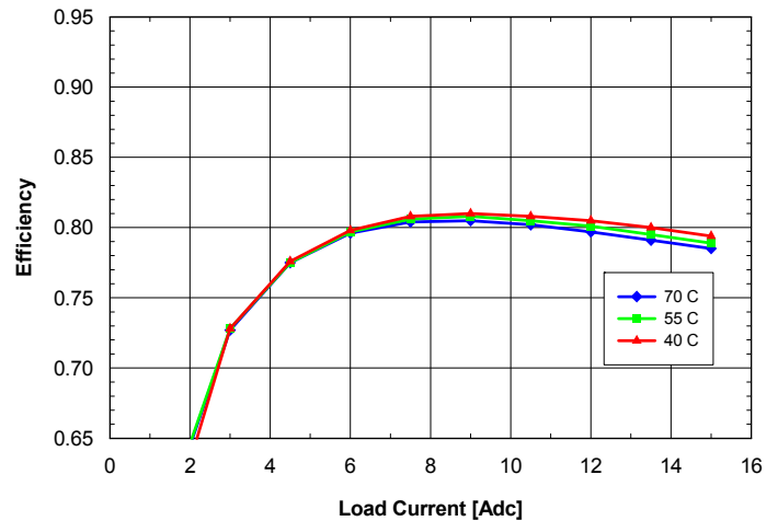
Fig. 1.0V.6: Efficiency vs. load current and ambient temperature for SQ24T/S15010 converter mounted vertically with V_{in} = 24\text{V} and air flowing from pin 3 to pin 1 at a rate of 200 LFM (1.0 m/s).
