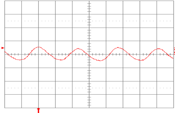
Fig. 3.3V.15: Input reflected ripple current, i_c (100 mA/div.), measured at input terminals at full rated load current and V_{in} = 24\ \text{V} . Refer to Fig. 3.3V.14 for test setup. Time scale: 1\ \mu\text{s}/\text{div} .
