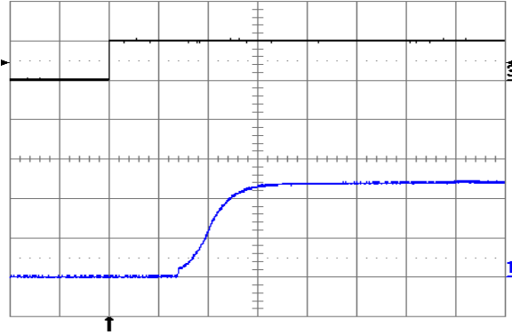
Fig. 12V.9: Turn-on transient at full rated load current (resistive) with no output capacitor at V_{in} = 24V , triggered via ON/OFF pin. Top trace: ON/OFF signal (5 V/div.). Bottom trace: output voltage (5 V/div.). Time scale: 1 ms/div.
