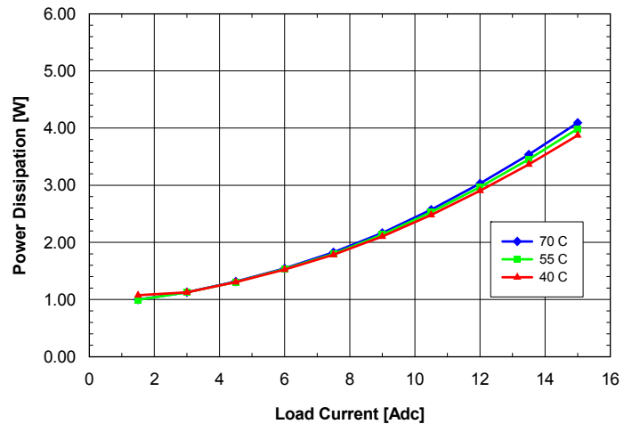
Fig. 1.0V.8: Power dissipation vs. load current and ambient temperature for SQ24T/S15010 converter mounted vertically with V_{in} = 24\text{V} and air flowing from pin 3 to pin 1 at a rate of 200 LFM (1.0 m/s).
