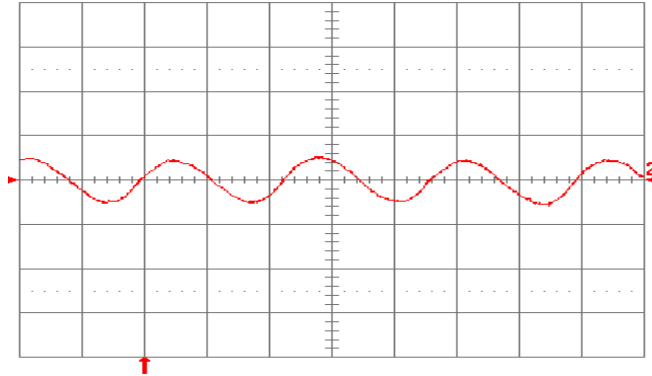
Fig. 12V.15: Input reflected ripple current, i_c (100 mA/div.), measured at input terminals at full rated load current and V_{in} = 24\ \text{V} . Refer to Fig. 12V.14 for test setup. Time scale: 1\ \mu\text{s}/\text{div} .
