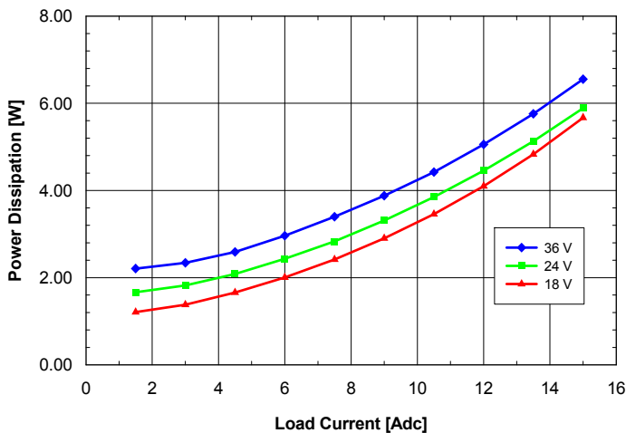
Fig. 2.5V.7: Power dissipation vs. load current and input voltage for SQ24T/S15025 converter mounted vertically with air flowing from pin 3 to pin 1 at a rate of 300 LFM (1.5 m/s) and T_a = 25^\circ\text{C} .
