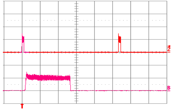
Fig. 12V.18: Load current (top trace, 5 A/div., 20 ms/div.) into a 10 mΩ short circuit during restart, at Vin = 24V. Bottom trace (5 A/div., 1 ms/div.) is an expansion of the on-time portion of the top trace.
