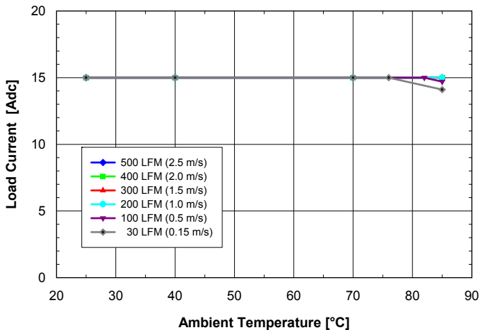
Fig. 1.5V.3: Available load current vs. ambient temperature and airflow rates for SQ24S15015 converter mounted vertically with V_{in} = 24V , air flowing from pin 3 to pin 1 and maximum FET temperature \leq 120^{\circ}C .
