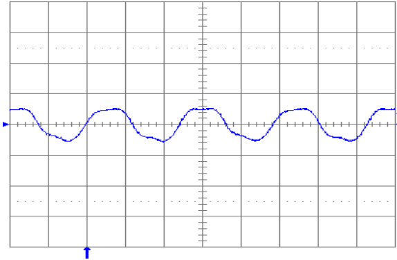
Fig. 6.0V.13: Output voltage ripple (50 mV/div.) at full rated load current into a resistive load with C_o = 10\ \mu\text{F} tantalum + 1\ \mu\text{F} ceramic and V_{in} = 24\ \text{V} . Time scale: 1\ \mu\text{s}/\text{div} .
