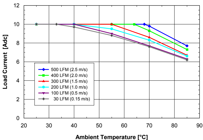
Fig. 5.0V.3: Available load current vs. ambient temperature and airflow rates for SQ24S10050 converter mounted vertically with V_{in} = 24V , air flowing from pin 3 to pin 1 and maximum FET temperature \leq 120^{\circ}C .
