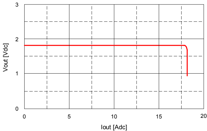
Fig. 1.8V.17: Output voltage vs. load current showing current limit point and converter shutdown point. Input voltage has almost no effect on current limit characteristic.
