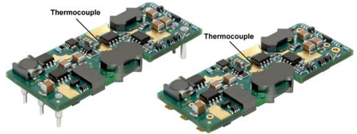
Fig. H: Location of the thermocouple for thermal testing.
