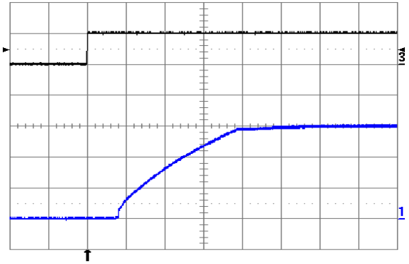
Fig. 6.0V.10: Turn-on transient at full rated load current (resistive) plus 10,000µF at V_{in} = 24V , triggered via ON/OFF pin. Top trace: ON/OFF signal (5 V/div.). Bottom trace: output voltage (2 V/div.). Time scale: 2 ms/div.
