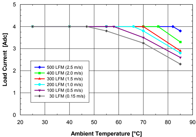
Fig. 12V.1: Available load current vs. ambient air temperature and airflow rates for SQ24T04120 converter with B height pins mounted vertically with V_{in} = 24V , air flowing from pin 3 to pin 1 and maximum FET temperature \leq 120^{\circ}C .
