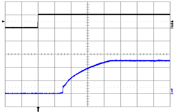
Fig. 2.5V.10: Turn-on transient at full rated load current (resistive) plus 10,000 \mu F at V_{in} = 24V , triggered via ON/OFF pin. Top trace: ON/OFF signal (5 V/div.). Bottom trace: output voltage (1 V/div.). Time scale: 1 ms/div.
