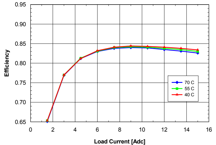
Fig. 1.5V.6: Efficiency vs. load current and ambient temperature for SQ24T/S15015 converter mounted vertically with V_{in} = 24\text{V} and air flowing from pin 3 to pin 1 at a rate of 200 LFM (1.0 m/s).
