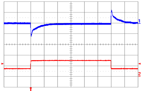
Fig. 2.0V.12: Output voltage response to load current step-change (3.75A – 7.5A – 3.75A) at V_{in} = 24V . Top trace: output voltage (100 mV/div.). Bottom trace: load current (5 A/div.). Current slew rate: 5 A/ \mu s . C_o = 450 \mu F tantalum + 1 \mu F ceramic. Time scale: 0.2 ms/div.
