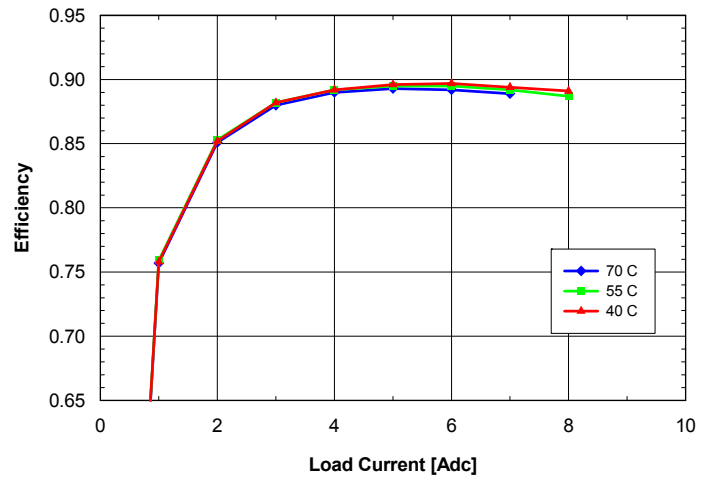
Fig. 6.0V.6: Efficiency vs. load current and ambient temperature for SQ24T/S08060 converter mounted vertically with V_{in} = 24\text{V} and air flowing from pin 3 to pin 1 at a rate of 200 LFM (1.0 m/s).
