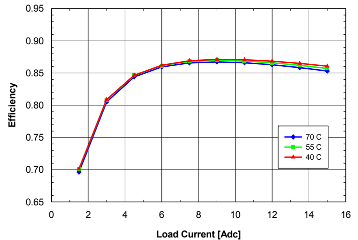
Fig. 2.5V.6: Efficiency vs. load current and ambient temperature for SQ24T/S15025 converter mounted vertically with V_{in} = 24\text{V} and air flowing from pin 3 to pin 1 at a rate of 200 LFM (1.0 m/s).
