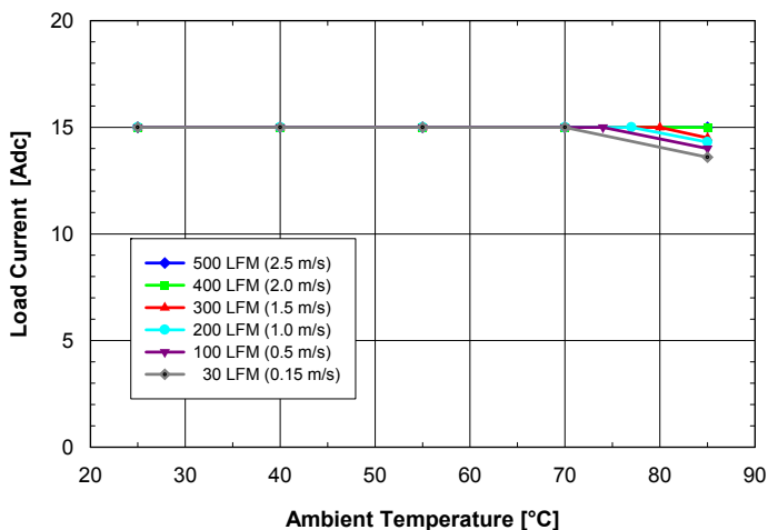
Fig. 1.8V.3: Available load current vs. ambient temperature and airflow rates for SQ24S15018 converter mounted vertically with V_{in} = 24V , air flowing from pin 3 to pin 1 and maximum FET temperature \leq 120^{\circ}C .
