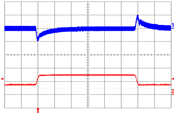
Fig. 1.0V.11: Output voltage response to load current step-change (3.75 A – 7.5 A – 3.75 A) at V_{in} = 24V . Top trace: output voltage (100 mV/div.). Bottom trace: load current (5 A/div.). Current slew rate: 0.1 A/µs. C_o = 1 \mu F ceramic. Time scale: 0.2 ms/div.
