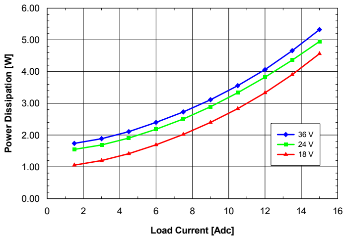
Fig. 1.8V.7: Power dissipation vs. load current and input voltage for SQ24T/S15018 converter mounted vertically with air flowing from pin 3 to pin 1 at a rate of 300 LFM (1.5 m/s) and T_a = 25^\circ\text{C} .
