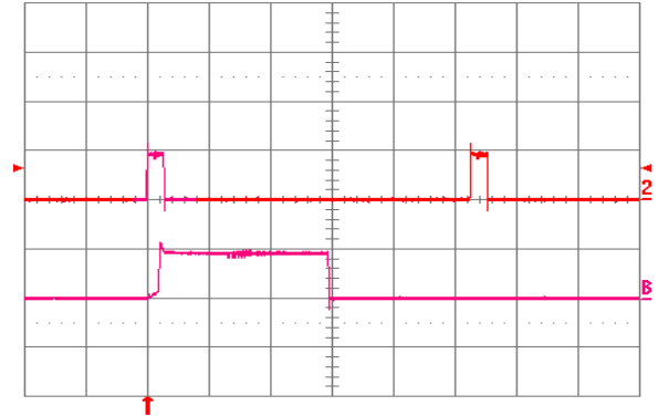
Fig. 1.8V.18: Load current (top trace, 20 A/div., 20 ms/div.) into a 10 mΩ short circuit during restart, at V_{in} = 24V . Bottom trace (20 A/div., 2 ms/div.) is an expansion of the on-time portion of the top trace.
