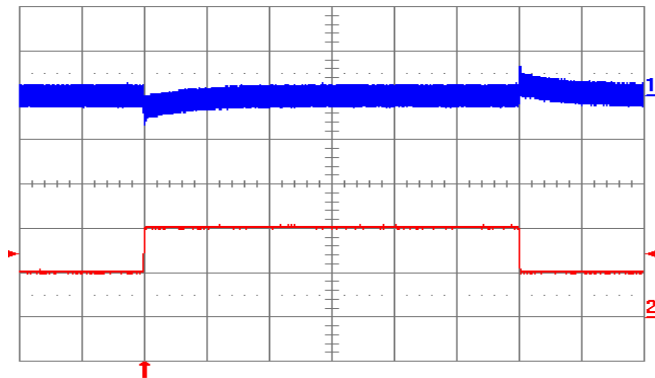
Fig. 12V.11: Output voltage response to load current step-change (1A – 2A – 1A) at V_{in} = 24V . Top trace: output voltage (200 mV/div.). Bottom trace: load current (1 A/div.). Current slew rate: 0.1 A/µs. C_o = 1 \mu F ceramic. Time scale: 0.5 ms/div.
