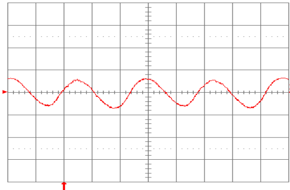
Fig. 6.0V.15: Input reflected ripple current, i_c (100 mA/div.), measured at input terminals at full rated load current and V_{in} = 24\ \text{V} . Refer to Fig. 6.0V.14 for test setup. Time scale: 1\ \mu\text{s}/\text{div} .
