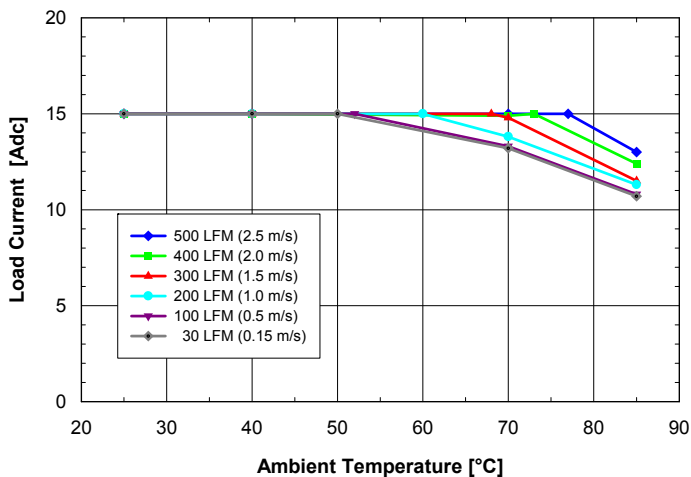
Fig. 3.3V.3: Available load current vs. ambient temperature and airflow rates for SQ24S15033 converter mounted vertically with V_{in} = 24V , air flowing from pin 3 to pin 1 and maximum FET temperature \leq 120^{\circ}C .
