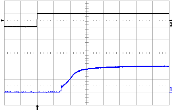
Fig. 2.0V.9: Turn-on transient at full rated load current (resistive) with no output capacitor at V_{in} = 24V , triggered via ON/OFF pin. Top trace: ON/OFF signal (5 V/div.). Bottom trace: output voltage (1 V/div.). Time scale: 1 ms/div.
