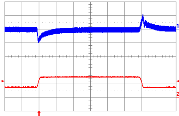
Fig. 2.0V.11: Output voltage response to load current step-change (3.75A – 7.5A – 3.75A) at V_{in} = 24V . Top trace: output voltage (100 mV/div.). Bottom trace: load current (5 A/div.). Current slew rate: 0.1 A/ \mu s . C_o = 1 \mu F ceramic. Time scale: 0.2 ms/div.
