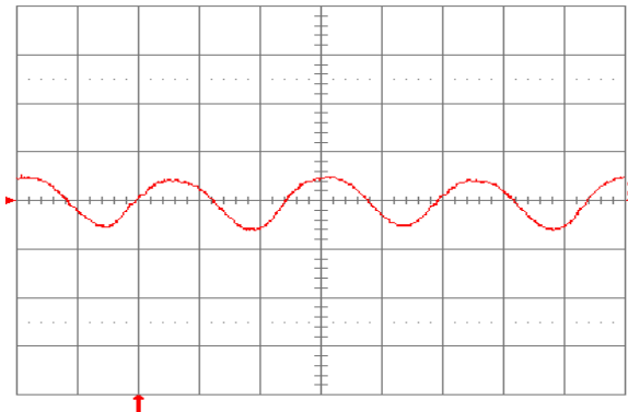
Fig. 2.0V.15: Input reflected ripple current, i_c (100 mA/div.), measured at input terminals at full rated load current and V_{in} = 24\ \text{V} . Refer to Fig. 2.0V.14 for test setup. Time scale: 1\ \mu\text{s}/\text{div} .
