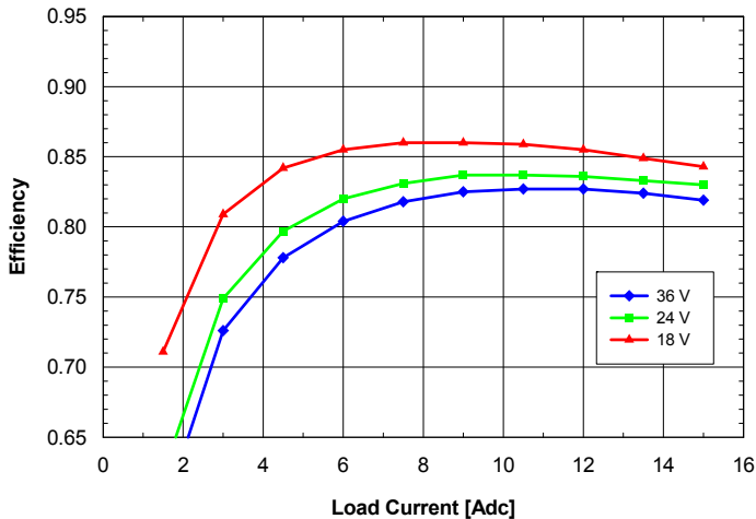
Fig. 1.5V.5: Efficiency vs. load current and input voltage for SQ24T/S15015 converter mounted vertically with air flowing from pin 3 to pin 1 at a rate of 300 LFM (1.5 m/s) and T_a = 25^\circ\text{C} .
