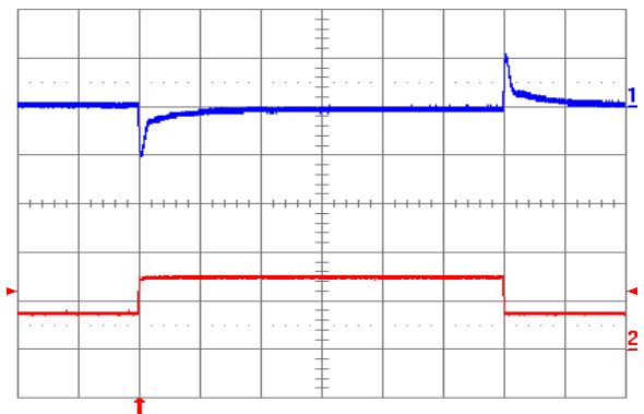
Fig. 1.8V.12: Output voltage response to load current step-change (3.75A – 7.5A – 3.75A) at V_{in} = 24V . Top trace: output voltage (100 mV/div.). Bottom trace: load current (5 A/div.). Current slew rate: 5 A/µs. C_o = 450 \mu F tantalum + 1 µF ceramic. Time scale: 0.2 ms/div.
