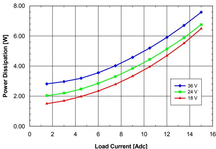
Fig. 3.3V.7: Power dissipation vs. load current and input voltage for SQ24T/S15033 converter mounted vertically with air flowing from pin 3 to pin 1 at a rate of 300 LFM (1.5 m/s) and T_a = 25^\circ\text{C} .
