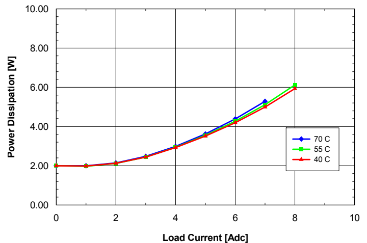
Fig. 6.0V.8: Power dissipation vs. load current and ambient temperature for SQ24T/S08060 converter mounted vertically with V_{in} = 24\text{V} and air flowing from pin 3 to pin 1 at a rate of 200 LFM (1.0 m/s).
