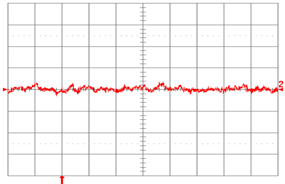
Fig. 1.2V.16: Input reflected ripple current, i_s (10 mA/div.), measured through 10 \mu\text{H} at the source at full rated load current and V_{in} = 24 \text{ V} . Refer to Fig. 1.2V.14 for test setup. Time scale: 1 \mu\text{s}/\text{div} .
