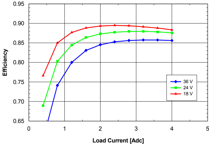
Fig. 12V.5: Efficiency vs. load current and input voltage for SQ24T/S04120 converter mounted vertically with air flowing from pin 3 to pin 1 at a rate of 300 LFM (1.5 m/s) and T_a = 25^\circ\text{C} .
