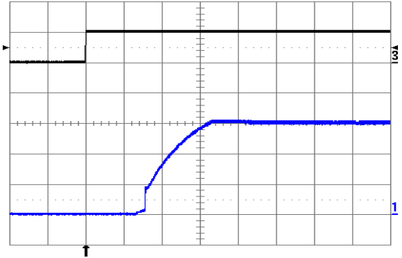
Fig. 1.5V.10: Turn-on transient at full rated load current (resistive) plus 10,000 \mu F at V_{in} = 24V , triggered via ON/OFF pin. Top trace: ON/OFF signal (5 V/div.). Bottom trace: output voltage (0.5 V/div.). Time scale: 1 ms/div.
