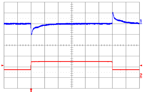
Fig. 3.3V.12: Output voltage response to load current step-change (3.75A – 7.5A – 3.75A) at V_{in} = 24V . Top trace: output voltage (100 mV/div.). Bottom trace: load current (5 A/div.). Current slew rate: 5 A/ \mu s . C_o = 450 \mu F tantalum + 1 \mu F ceramic. Time scale: 0.2 ms/div.
