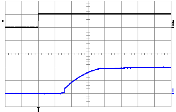
Fig. 2.0V.10: Turn-on transient at full rated load current (resistive) plus 10,000 \mu F at V_{in} = 24V , triggered via ON/OFF pin. Top trace: ON/OFF signal (5 V/div.). Bottom trace: output voltage (1 V/div.). Time scale: 1 ms/div.
