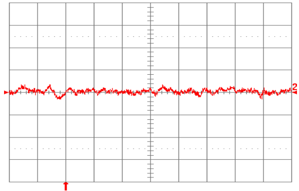
Fig. 2.5V.16: Input reflected ripple current, i_s (10 mA/div.), measured through 10\ \mu\text{H} at the source at full rated load current and V_{in} = 24\ \text{V} . Refer to Fig. 2.5V.14 for test setup. Time scale: 1\ \mu\text{s}/\text{div} .
