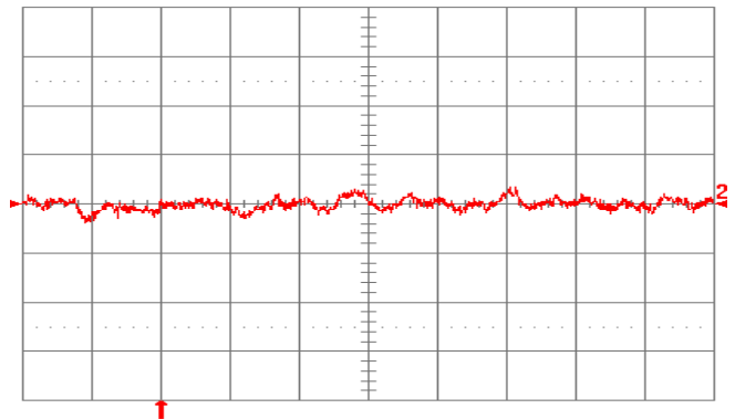
Fig. 12V.16: Input reflected ripple current, i_s (10 mA/div.), measured through 10\ \mu\text{H} at the source at full rated load current and V_{in} = 24\ \text{V} . Refer to Fig. 12V.14 for test setup. Time scale: 1\ \mu\text{s}/\text{div} .
