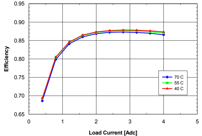
Fig. 12V.6: Efficiency vs. load current and ambient temperature for SQ24T/S04120 converter mounted vertically with V_{in} = 24\text{V} and air flowing from pin 3 to pin 1 at a rate of 200 LFM (1.0 m/s).
