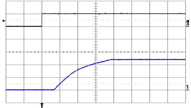
Fig. 12V.10: Turn-on transient at full rated load current (resistive) plus 1,000µF at V_{in} = 24V , triggered via ON/OFF pin. Top trace: ON/OFF signal (5 V/div.). Bottom trace: output voltage (5 V/div.). Time scale: 2 ms/div.
