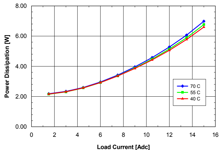
Fig. 3.3V.8: Power dissipation vs. load current and ambient temperature for SQ24T/S15033 converter mounted vertically with V_{in} = 24\text{V} and air flowing from pin 3 to pin 1 at a rate of 200 LFM (1.0 m/s).
