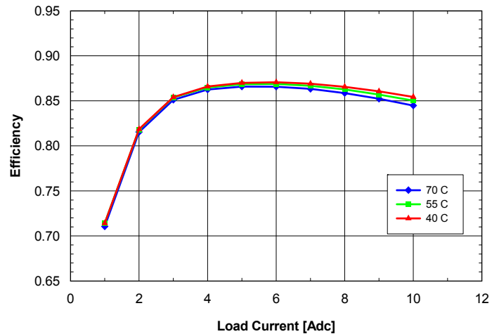
Fig. 5.0V.6: Efficiency vs. load current and ambient temperature for SQ24T/S10050 converter mounted vertically with V_{in} = 24\text{V} and air flowing from pin 3 to pin 1 at a rate of 200 LFM (1.0 m/s).
