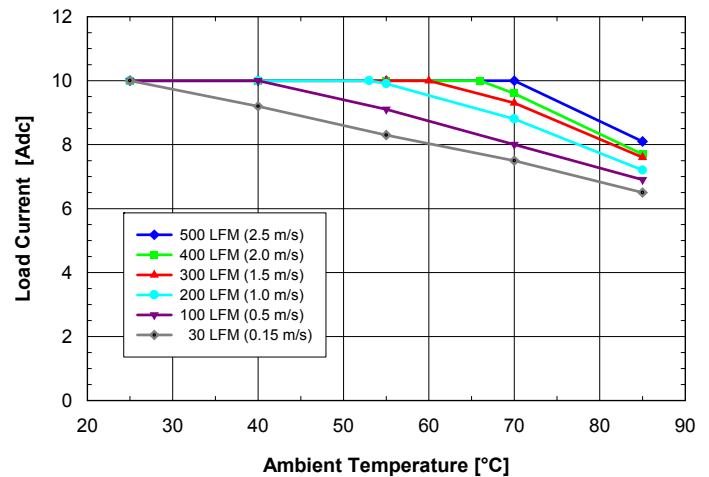
Fig. 5.0V.4: Available load current vs. ambient temperature and airflow rates for SQ24S10050 converter mounted horizontally with V_{in} = 24V , air flowing from pin 3 to pin 1 and maximum FET temperature \leq 120^{\circ}C .
