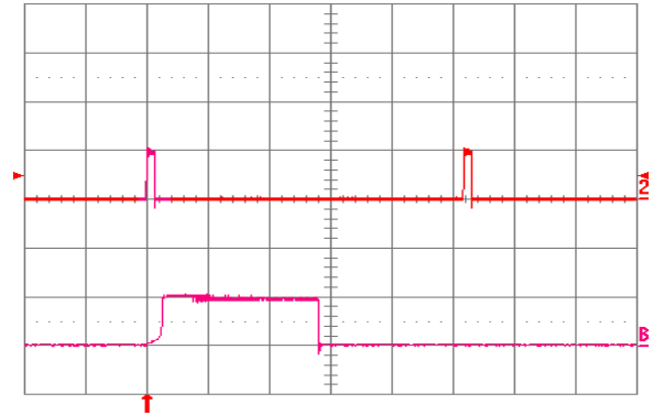
Fig. 3.3V.18: Load current (top trace, 20 A/div., 20 ms/div.) into a 10 mΩ short circuit during restart, at Vin = 24V. Bottom trace (20 A/div., 1 ms/div.) is an expansion of the on-time portion of the top trace.
