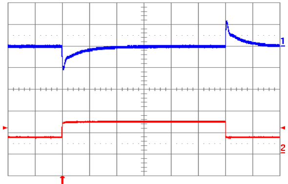
Fig. 1.2V.12: Output voltage response to load current step-change (3.75 A – 7.5 A – 3.75 A) at V_{in} = 24V . Top trace: output voltage (100 mV/div.). Bottom trace: load current (5 A/div.). Current slew rate: 5 A/ \mu s . C_o = 450 \mu F tantalum + 1 \mu F ceramic. Time scale: 0.2 ms/div.
