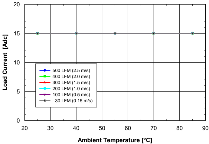
Fig. 1.2V.1: Available load current vs. ambient air temperature and airflow rates for SQ24T15012 converter with B height pins mounted vertically with V_{in} = 24V , air flowing from pin 3 to pin 1 and maximum FET temperature \leq 120^{\circ}C .
