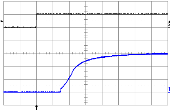
Fig. 6.0V.9: Turn-on transient at full rated load current (resistive) with no output capacitor at V_{in} = 24V , triggered via ON/OFF pin. Top trace: ON/OFF signal (5 V/div.). Bottom trace: output voltage (2 V/div.). Time scale: 1 ms/div.
