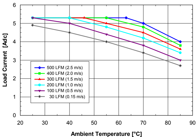
Fig. 8.0V.1: Available load current vs. ambient air temperature and airflow rates for SQ24T05080 converter with D height pins mounted vertically with V_{in} = 24\text{ V} , air flowing from pin 3 to pin 1 and maximum FET temperature \leq 120^\circ\text{C} .
