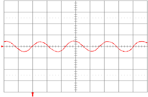
Fig. 2.5V.15: Input reflected ripple current, i_c (100 mA/div.), measured at input terminals at full rated load current and V_{in} = 24\ \text{V} . Refer to Fig. 2.5V.14 for test setup. Time scale: 1\ \mu\text{s}/\text{div} .
