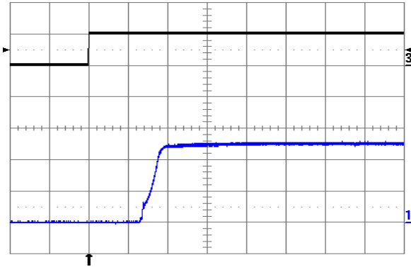
Fig. 2.5V.9: Turn-on transient at full rated load current (resistive) with no output capacitor at V_{in} = 24V , triggered via ON/OFF pin. Top trace: ON/OFF signal (5 V/div.). Bottom trace: output voltage (1 V/div.). Time scale: 1 ms/div.
