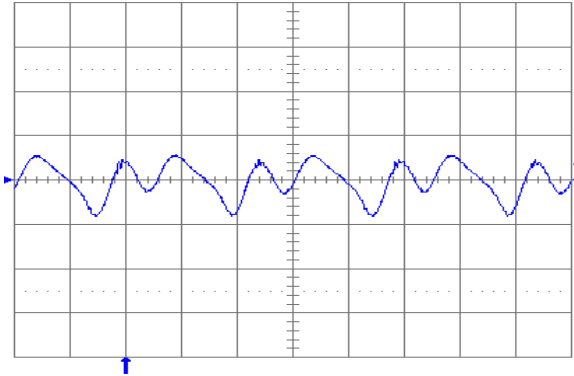
Fig. 1.0V.13: Output voltage ripple (20 mV/div.) at full rated load current into a resistive load with C_o = 10\ \mu\text{F} tantalum + 1\ \mu\text{F} ceramic and V_{in} = 24\ \text{V} . Time scale: 1\ \mu\text{s}/\text{div} .
