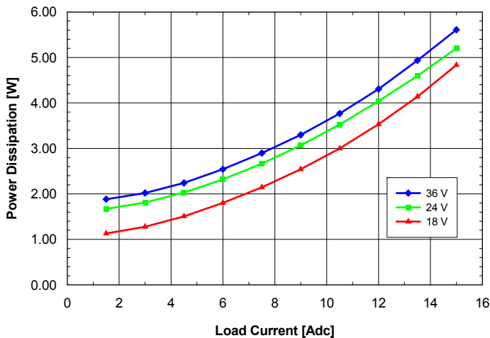
Fig. 2.0V.7: Power dissipation vs. load current and input voltage for SQ24T/S15020 converter mounted vertically with air flowing from pin 3 to pin 1 at a rate of 300 LFM (1.5 m/s) and T_a = 25^\circ\text{C} .
