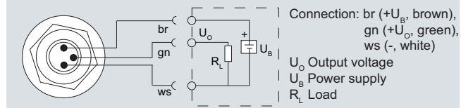
Connection with voltage output and cable
