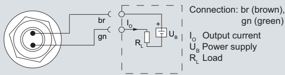
Connection with current output and cable
