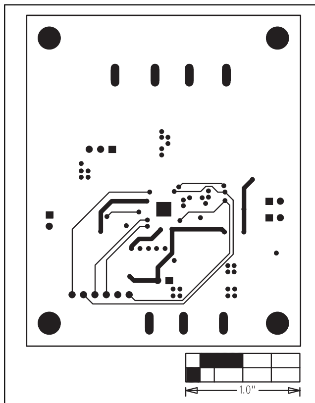
Figure 5. MAX5072 EV Kit PC Board Layout—Inner Trace Layer 3
