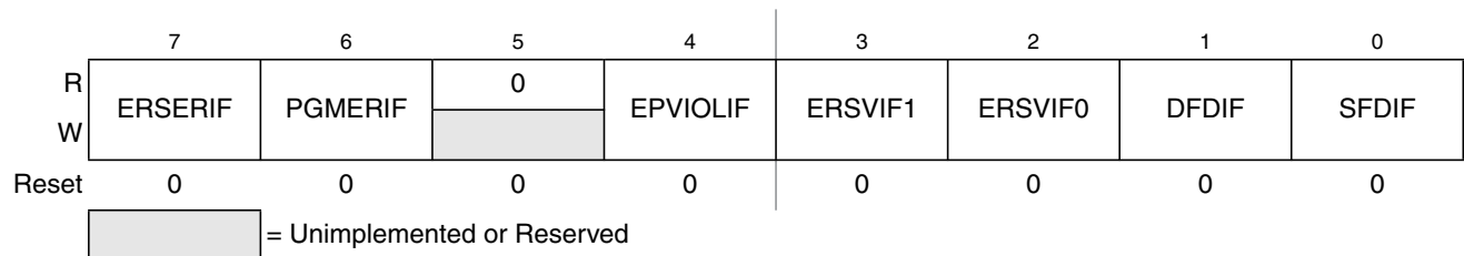
Figure 27-12. Flash Error Status Register (FERSTAT)
