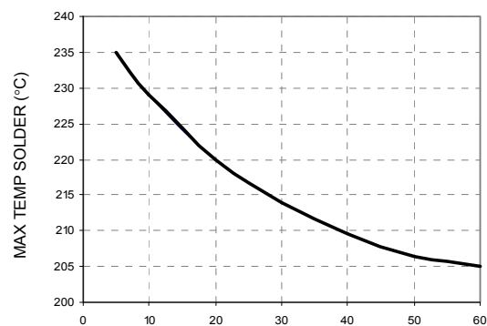
Figure 48. Time Limit Curve Above 205°C for Tin/Lead (Sn/Pb) process
