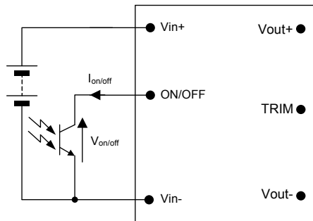
Figure 40. Remote On/Off Implementation.
