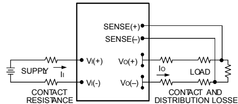
Figure 41. Circuit Configuration for remote sense .
