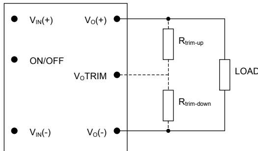
Figure 42. Circuit Configuration to Trim Output Voltage.
