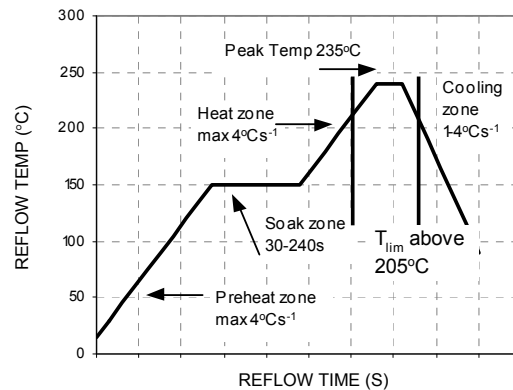
Figure 47. Reflow Profile for Tin/Lead (Sn/Pb) process
