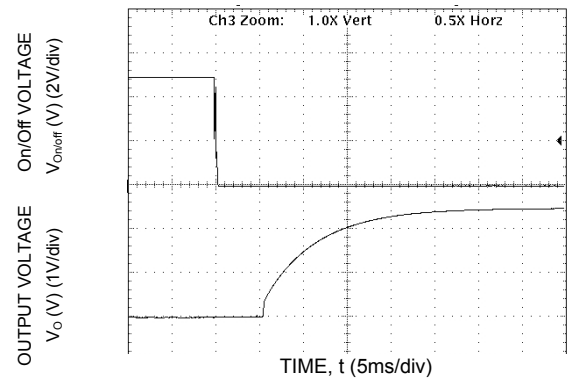
Figure 17. Typical Start-up Using Remote On/Off, negative logic version shown ( V_{IN} = V_{IN,NOM} , I_o = I_{o,max} ).
