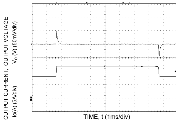
Figure 9. Transient Response to Dynamic Load Change from 50% to 75% to 50% of full load.
