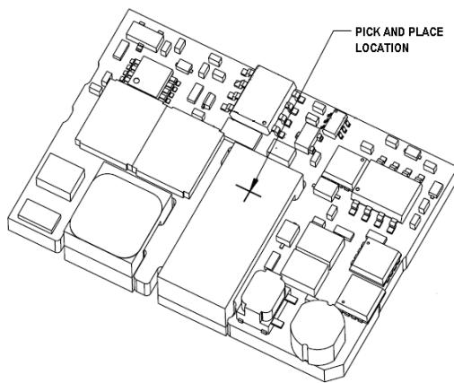
Figure 46. Pick and Place Location.
