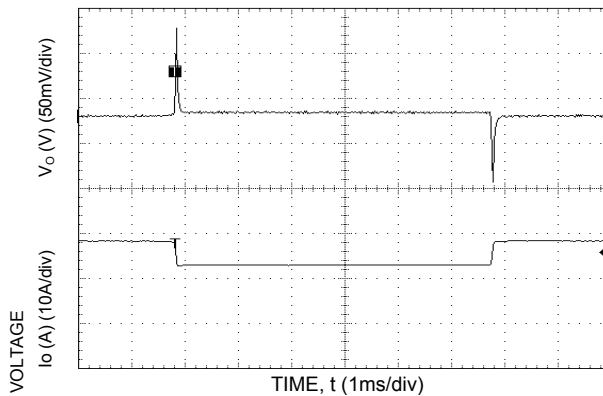
Figure 33. Transient Response to Dynamic Load Change from 75% to 50% to 75% of full load.
