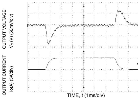
Figure 15. Transient Response to Dynamic Load Change from 50% to 75% to 50% of full load.
