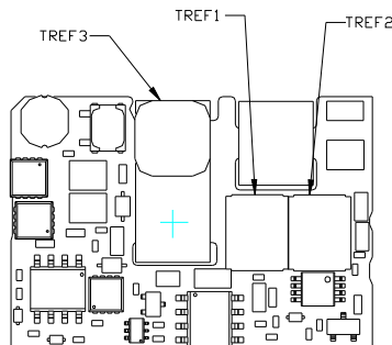
Figure 43. T_{ref} Temperature Measurement Locations.
