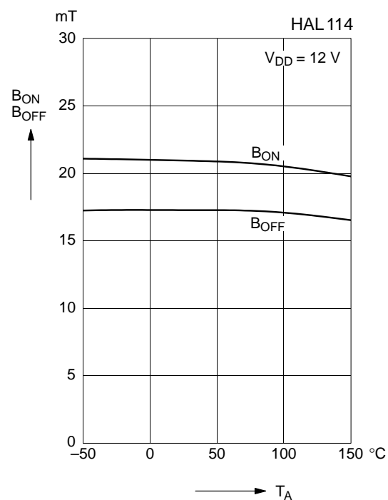
Fig. 4-4: Typical magnetic switching points versus temperature
