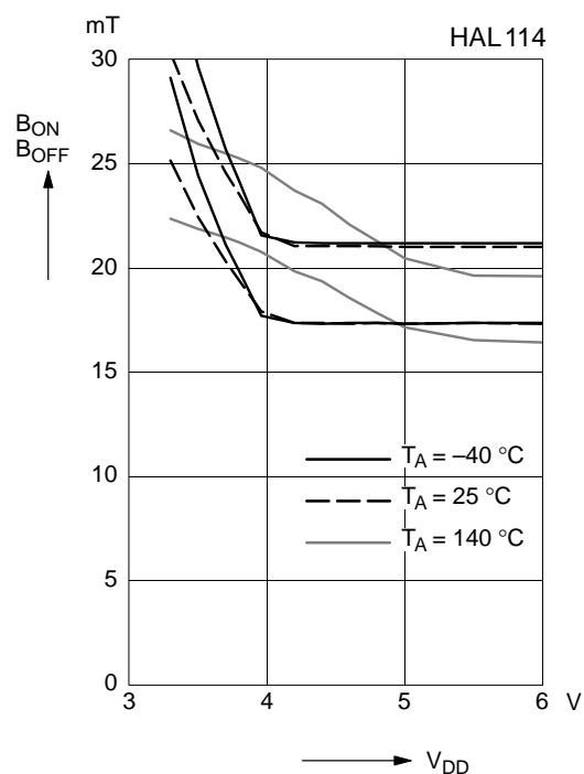
Fig. 4-3: Typical magnetic switching points versus supply voltage
