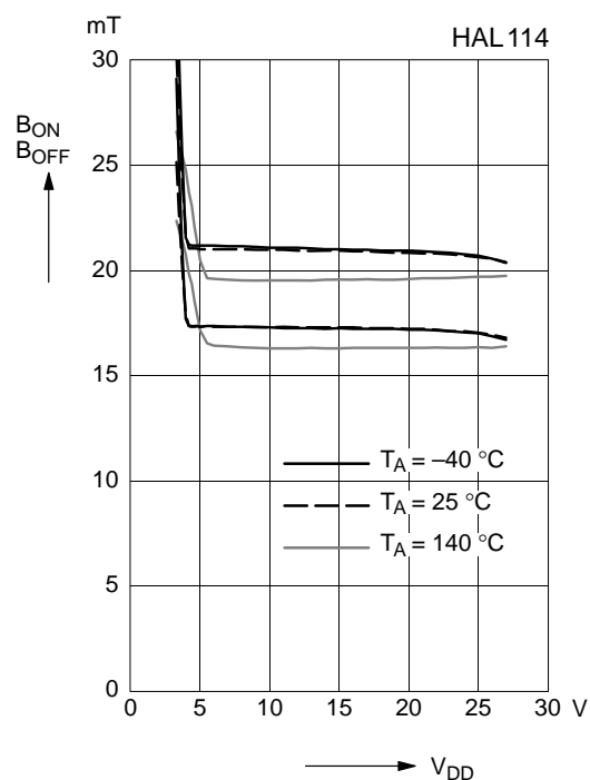
Fig. 4-2: Typical magnetic switching points versus supply voltage
