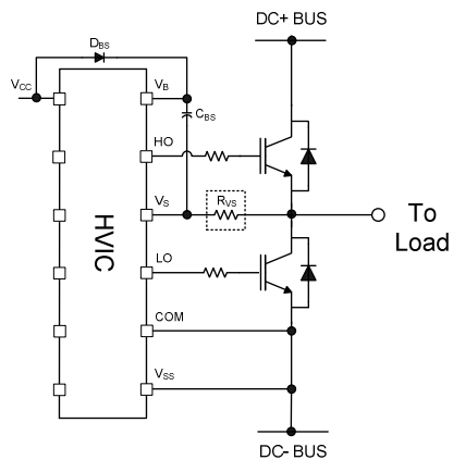
Figure 36: V S resistor
