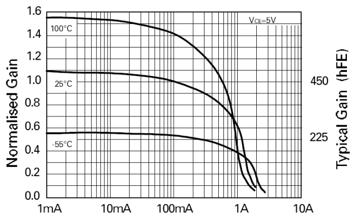
Collector Current h_{FE} vs I_C
