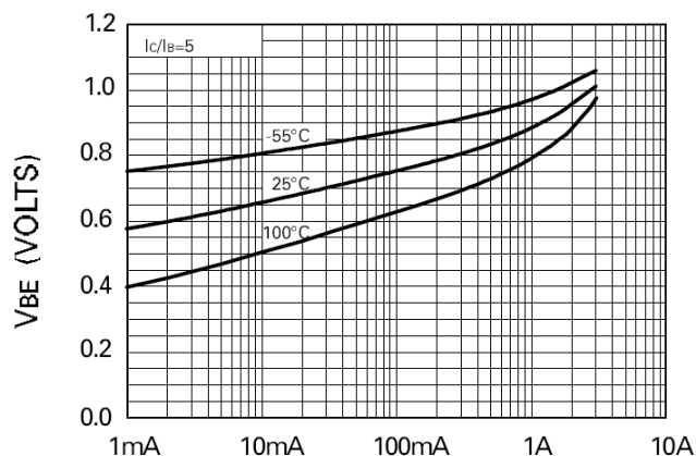
Collector Current V_{BE(SAT)} vs I_C
