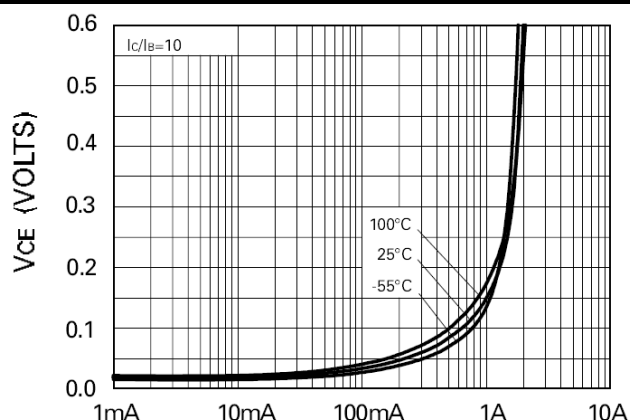
Collector Current V_{CE(SAT)} vs I_C
