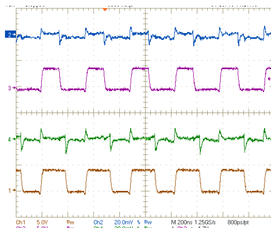
FIGURE 6. DCD OUTPUT RIPPLE ( V_{IN} = 4.2V , FULL LOADING @ VODCD1 AND VODCD2, TIME SCALE = 200ns) CH1: SW1 (5V/DIV), CH2: VODCD1 (20mV/DIV), CH3: SW2 (5V/DIV), CH4: VODCD2 (20mV/DIV)
