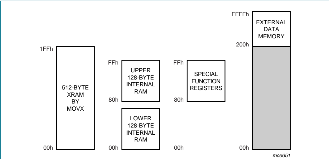
Fig 9. Internal and external data memory address space with EXTRAM = 0
