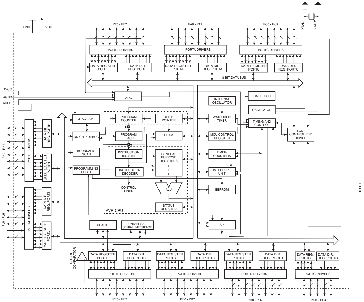
Figure 2-1. Block Diagram
