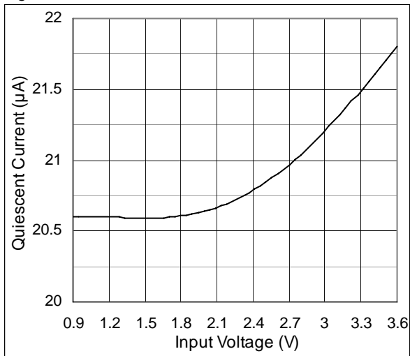
Figure 19. Quiescent Current vs. V_{CC}
