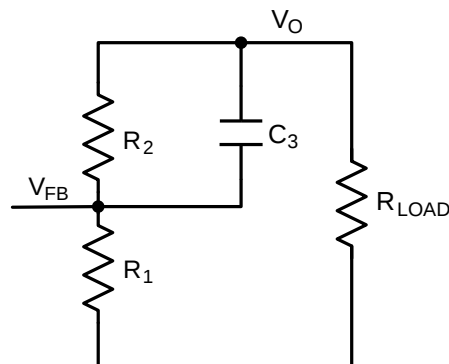
Figure 20. Setting Vout
