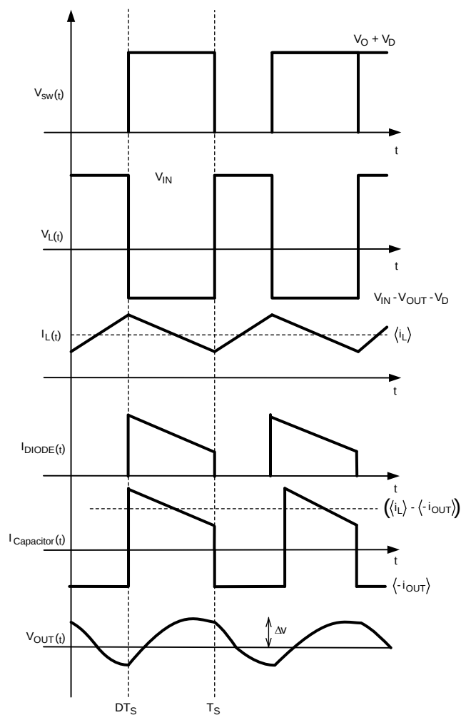
Figure 14. Typical Waveforms
