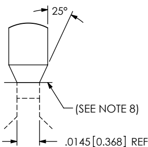
DETAIL 'A' SCALE 16:1
