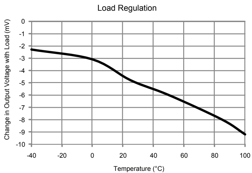
Figure 2-47 • Load Regulation
