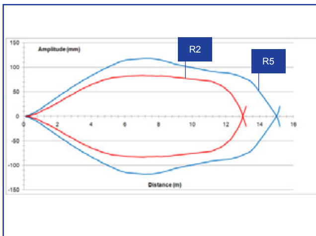
Polarized retroreflex on R2 and R5 reflectors
