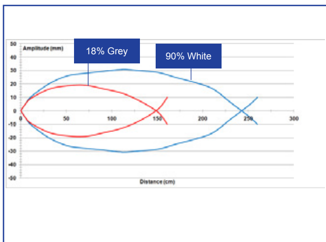
Diffused proximity
