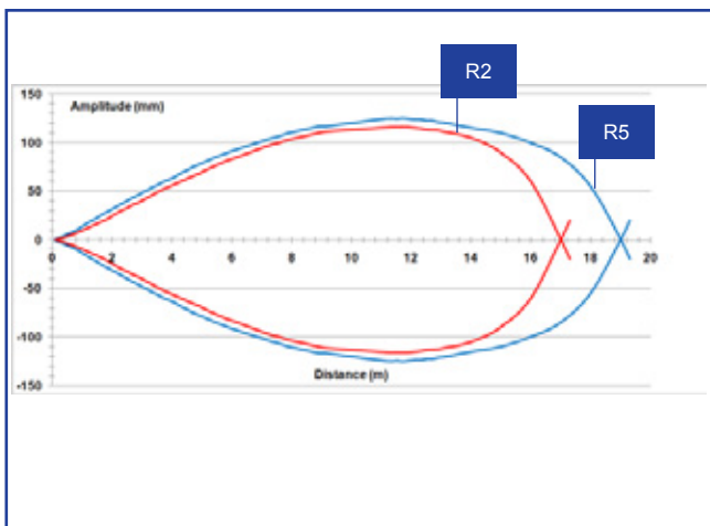
Retroreflex on R2 and R5 reflectors
