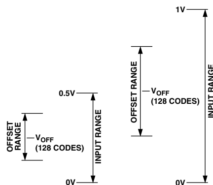
Figure 9. Relationship of Offset Range to Input Range
