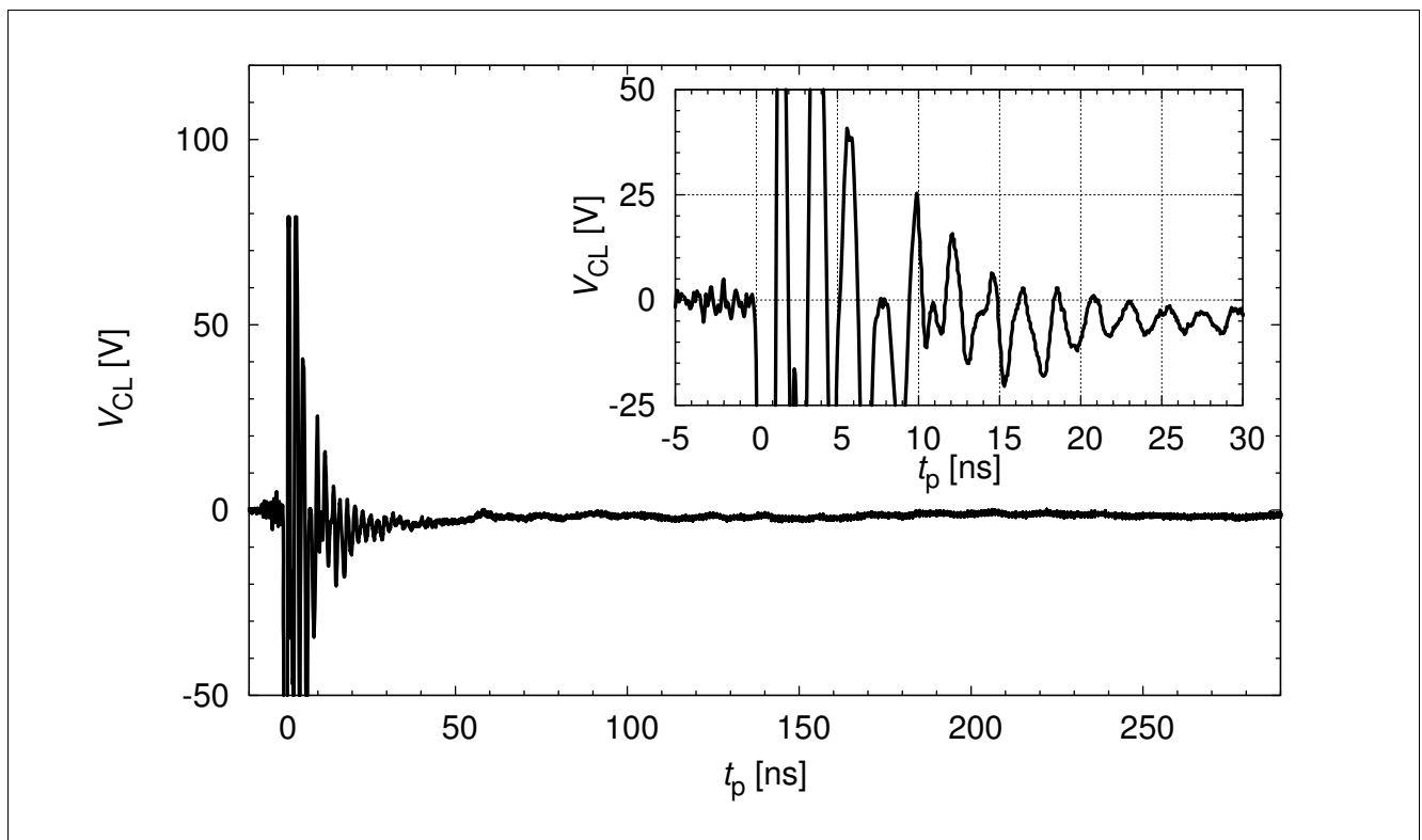
Figure 3-12 Clamping voltage at -15 kV contact discharge according IEC61000-4-2 ( R = 330 \, \Omega , C = 150 \, \text{pF} )
