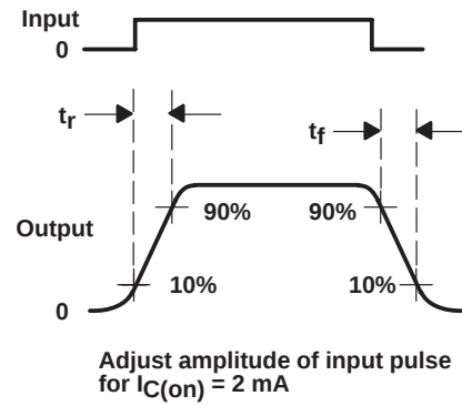
VOLTAGE WAVEFORMS
