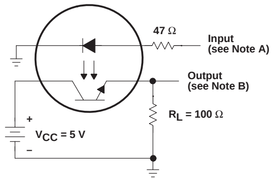
TEST CIRCUIT
