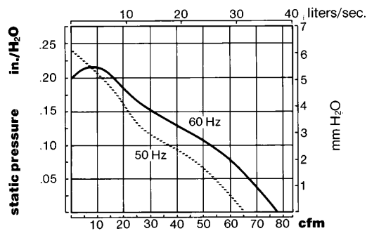
98XH Performance Curve
