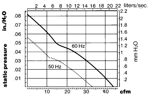
98XC Performance Curve
