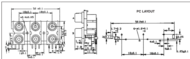
PHS-16B PCB mounting 6-way RCA Phono connector. Several different coloured inserts available. Nickel Silver or Gold plated finish. PHS-16B (Various)
