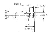
PC LAYOUT
