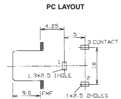
PC LAYOUT
