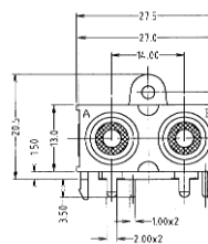
PHS-10A PCB mounting RCA Phono connector. Several different coloured inserts available. Nickel Silver or Gold plated finish. PHS-10A (Various)
