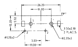
PC LAYOUT
