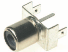
PHS-7A Vertical PCB mounting RCA Phono connector. Several different coloured inserts available. Nickel Silver or Gold plated finish. PHS-7A (FC68400)
