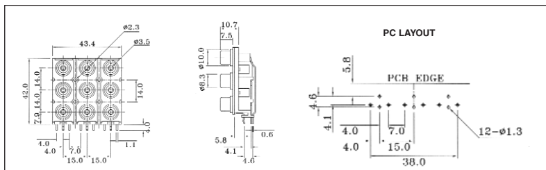
PHS-19A PCB mounting 9-way RCA Phono connector. Several different coloured inserts available. Nickel Silver or Gold plated finish. PHS-19A (Various)
