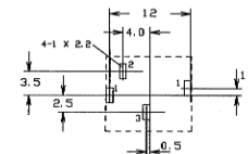
PC LAYOUT
