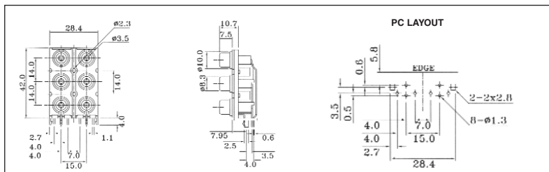
PHS-16C PCB mounting 6-way RCA Phono connector. Several different coloured inserts available. Nickel Silver or Gold plated finish. PHS-16C (Various)
