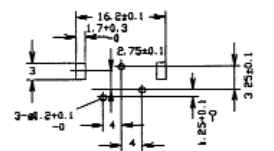
PC LAYOUT
