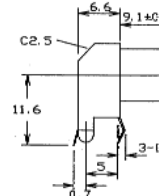
PHS-6A PCB mounting RCA Phono connector. Several different coloured inserts available. Nickel Silver or Gold plated finish. PHS-6A (Various)
