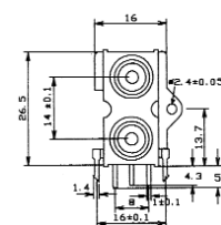
PHS-10B PCB mounting dual RCA Phono connector. Several different coloured inserts available. Nickel Silver or Gold plated finish. PHS-10B (Various)
