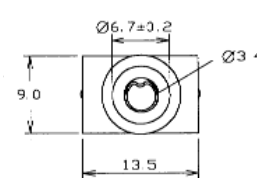
PHS-7A Vertical PCB mounting RCA Phono connector. Several different coloured inserts available. Nickel Silver or Gold plated finish. PHS-7A (FC68400)
