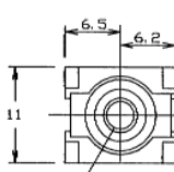
PHS-4B Snap In PCB mounting RCA Phono connector. Only available with black insert. PHS-4B (FC68375)
