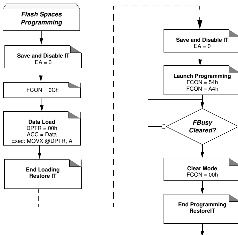
Figure 23. Hardware Programming Procedure
