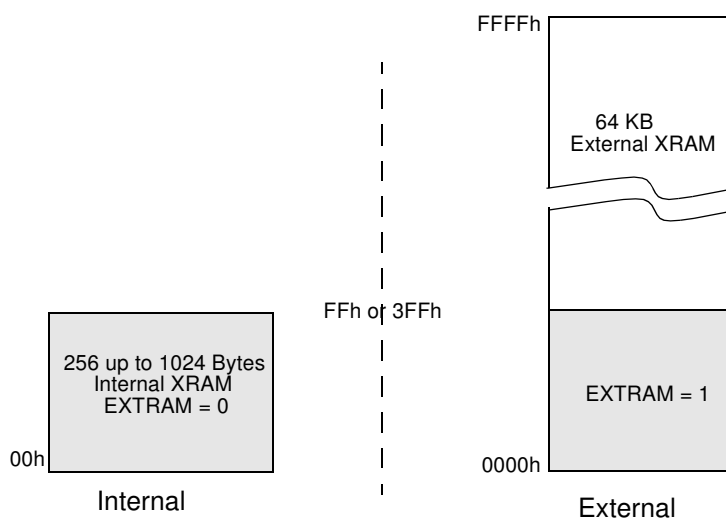
Figure 11. Internal and External Data Memory Organization XRAM-XRAM
