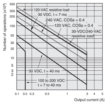
Durability Curve
