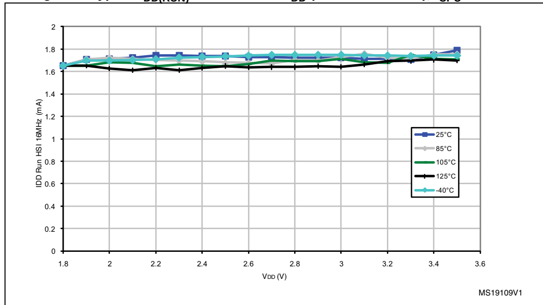
Figure 9. Typical I_{DD(RUN)} from RAM vs. V_{DD} (HSI clock source), f_{CPU} = 16 MHz
