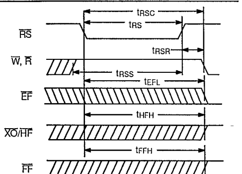
Figure 2. Reset Timing
