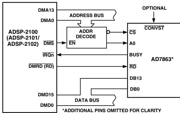
Figure 14. AD7863-ADSP-2100 Interface
