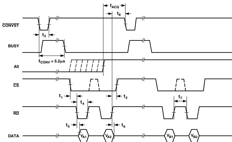
Figure 1. Timing Diagram
