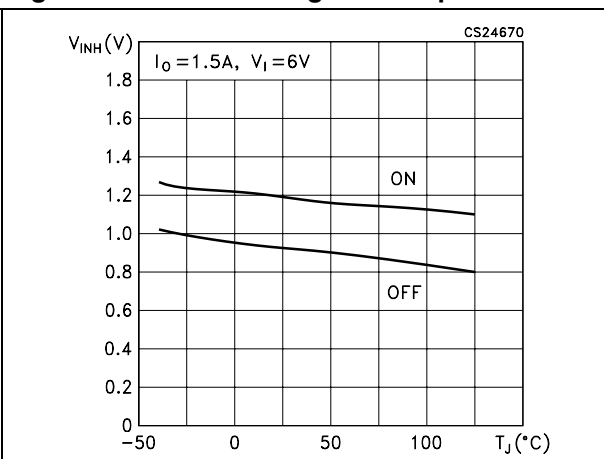
Figure 16. Inhibit voltage vs. temperature
