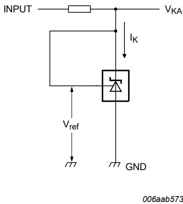
Fig. 5. Test circuit to Figures 3 and 4
