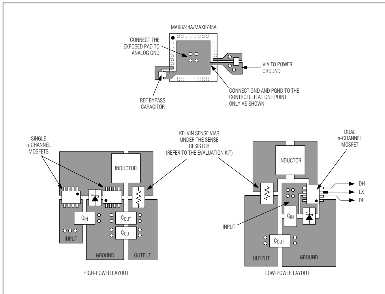
Figure 9. PCB Layout
