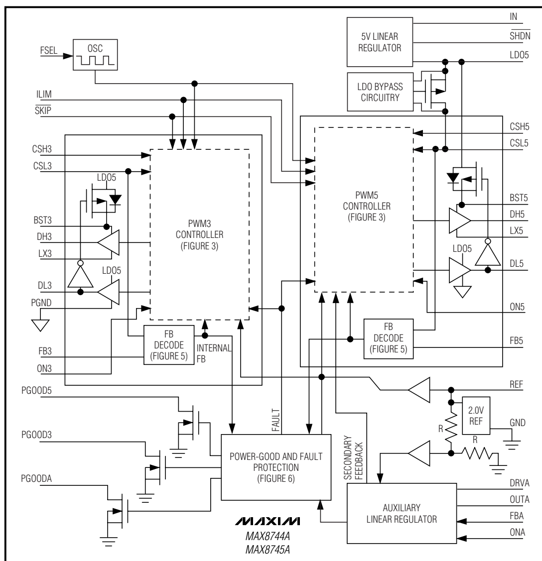
Figure 2. Block Diagram
