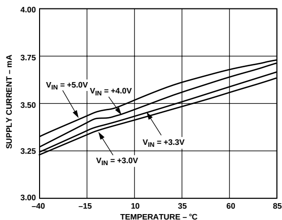
Figure 5. Supply Current vs. Temperature in Normal Mode
