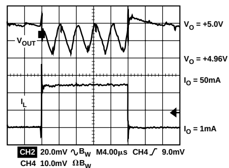
Figure 13. Load Transient Response Based on Circuit of Figure 1
