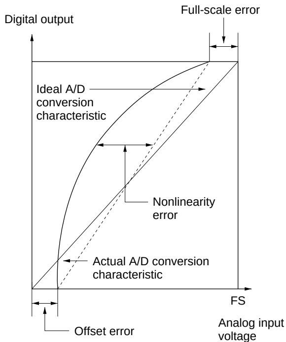
Figure 15.9 A/D Conversion Accuracy Definitions (2)
