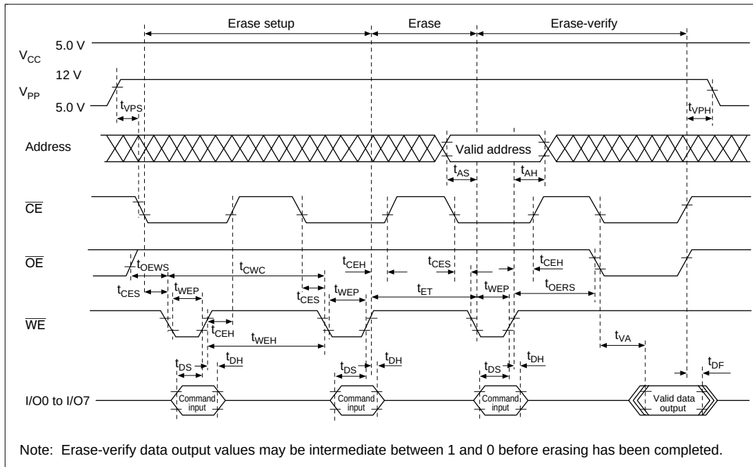
Figure 20.19 Erase Timing
