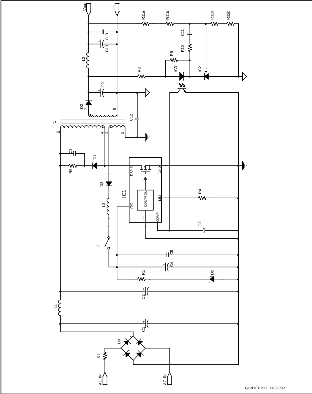
Figure 1: Application schematic
