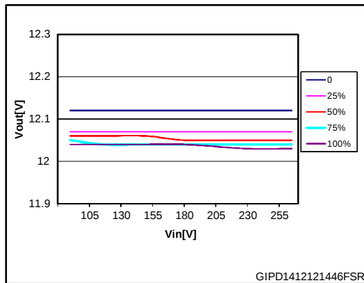
Figure 9: Line regulation
