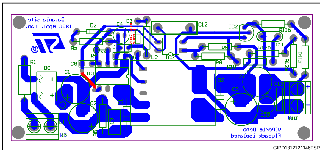
Figure 2: Board layout
