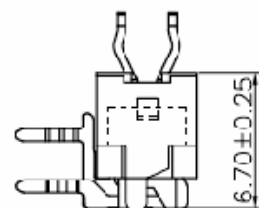
Mating Height Draw.
