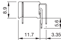
Dimensions [mm] for Part No. 19-940
